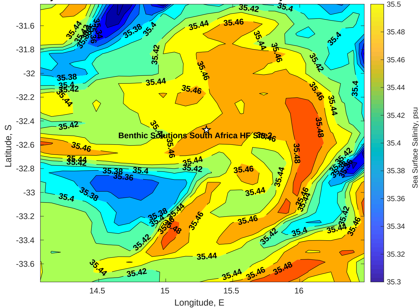
Surface Salinity for Benthic Solutions South Africa HF Site2 at 10-May-2025 00:00:00
