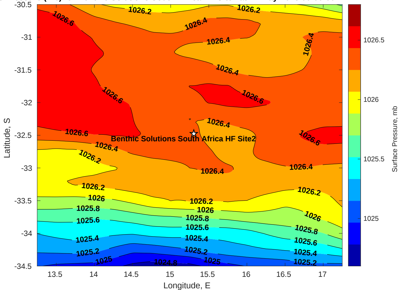
Surface Pressure (mb) for Benthic Solutions South Africa HF Site2 at 12-May-2025 00:00:00
