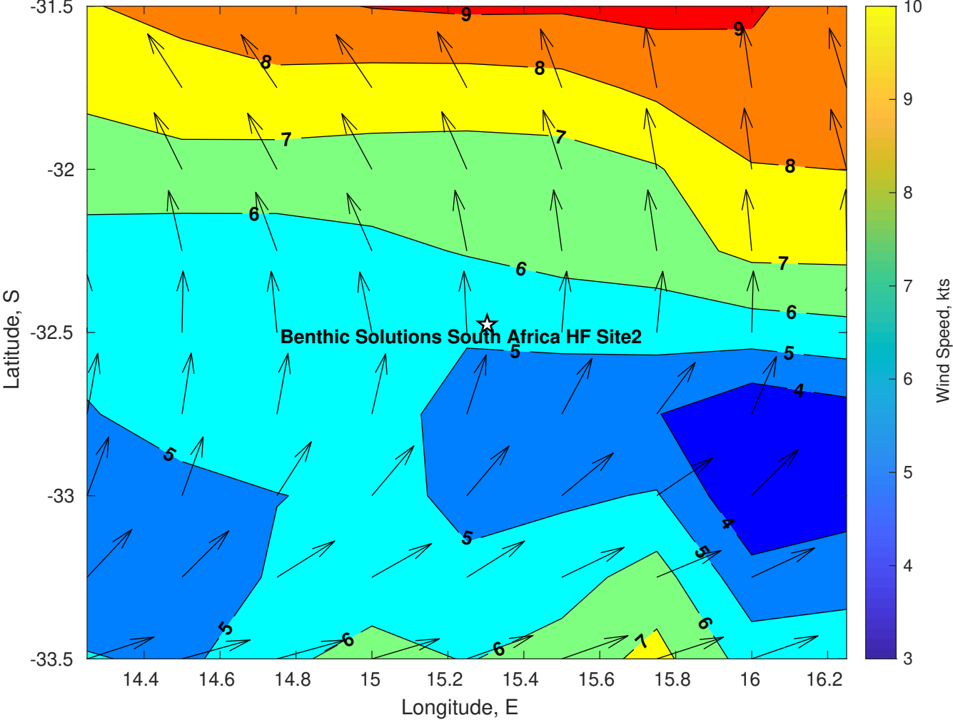
Winds (kts) for Benthic Solutions South Africa HF Site2 at 11-May-2025 09:00:00
