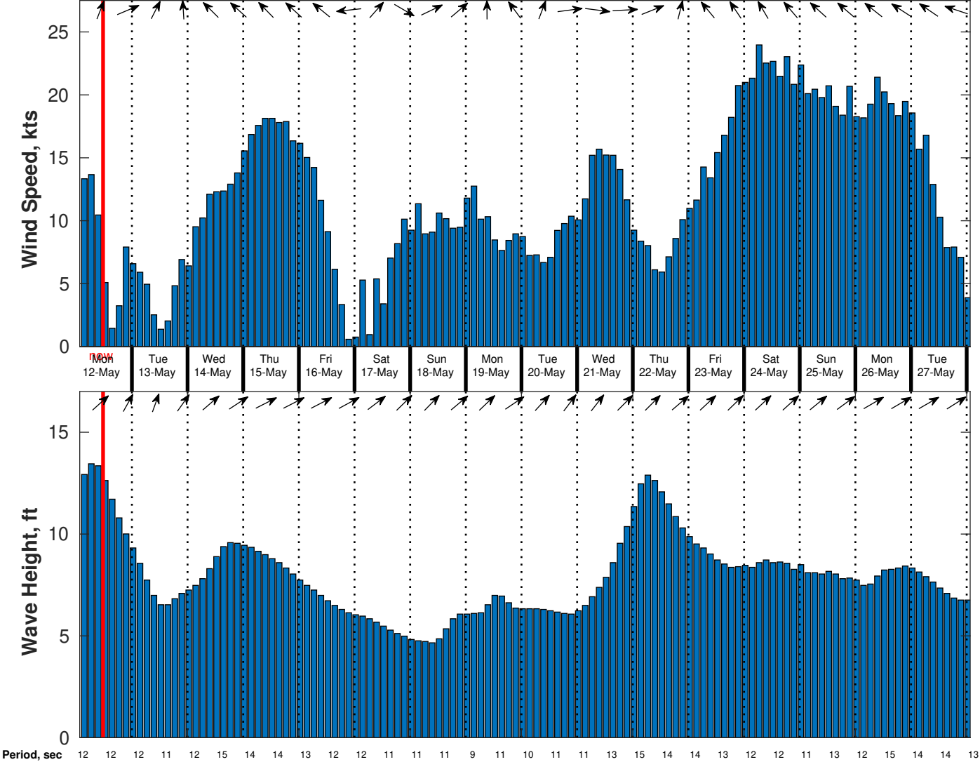
Wind & Wave Forecast for Benthic Solutions South Africa HF Site2 from 11-May-2025 02:00:00 to 27-May-2025 02:00:00
