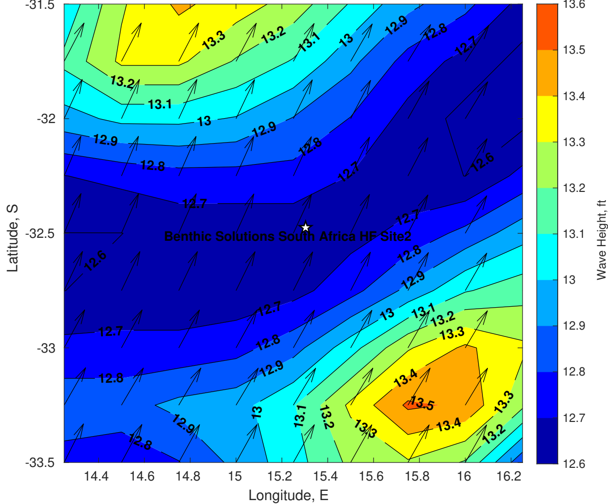
Wave Height (ft) for Benthic Solutions South Africa HF Site2 at 11-May-2025 09:00:00
