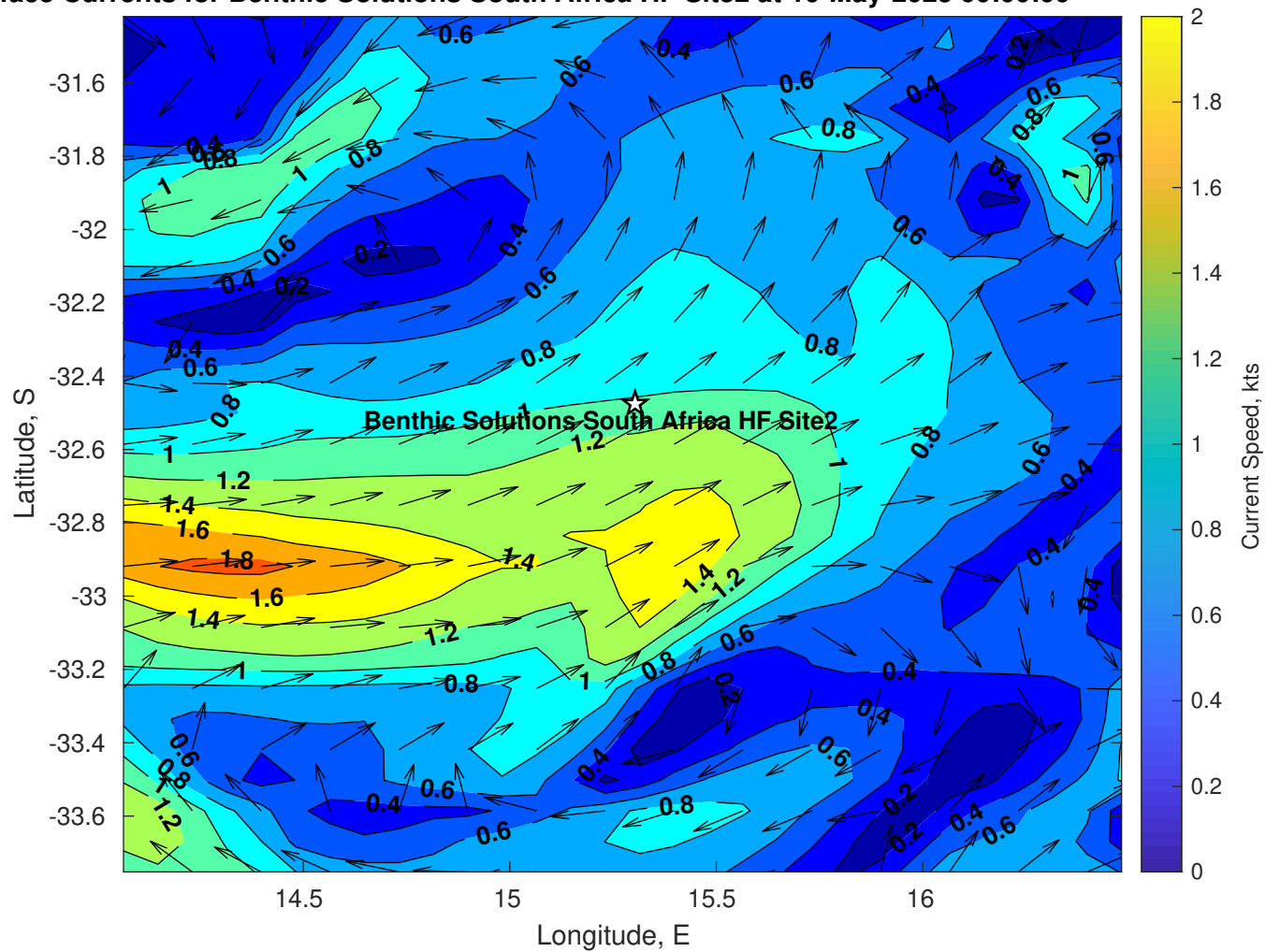
Surface Currents for Benthic Solutions South Africa HF Site2 at 10-May-2025 00:00:00
