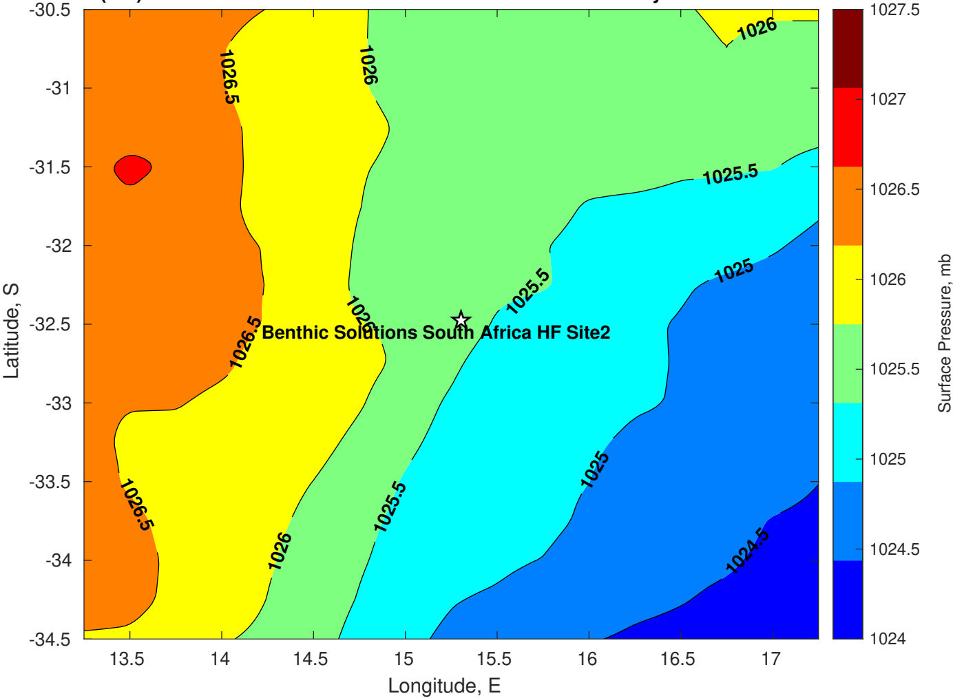
Surface Pressure (mb) for Benthic Solutions South Africa HF Site2 at 11-May-2025 00:00:00
