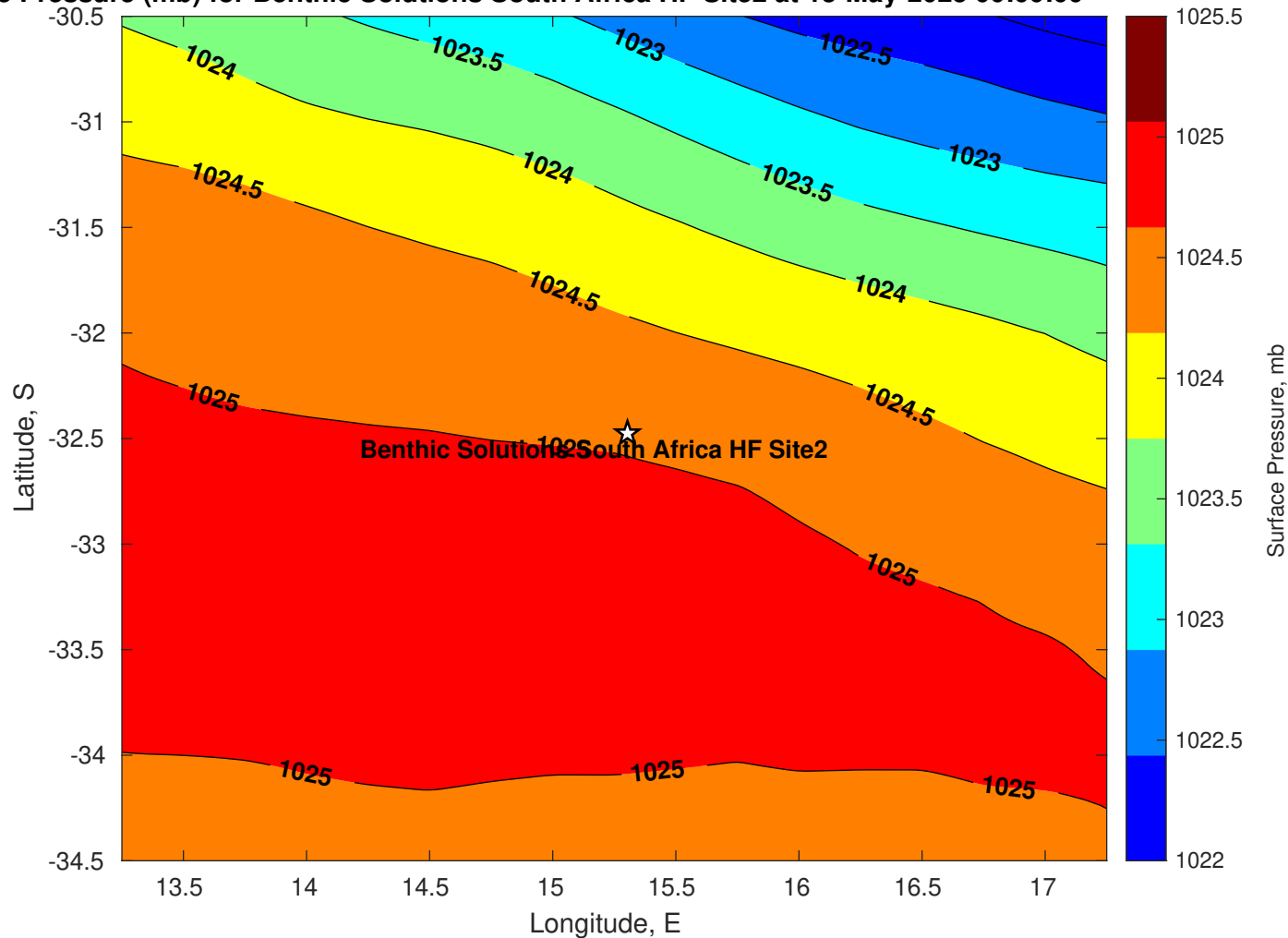
Surface Pressure (mb) for Benthic Solutions South Africa HF Site2 at 13-May-2025 00:00:00
