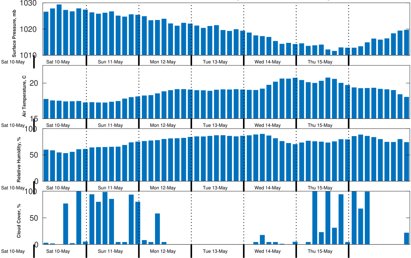
Met Forecast for Benthic Solutions South Africa HF Site2 from 11-May-2025 00:00:00 to 18-May-2025 00:00:00
