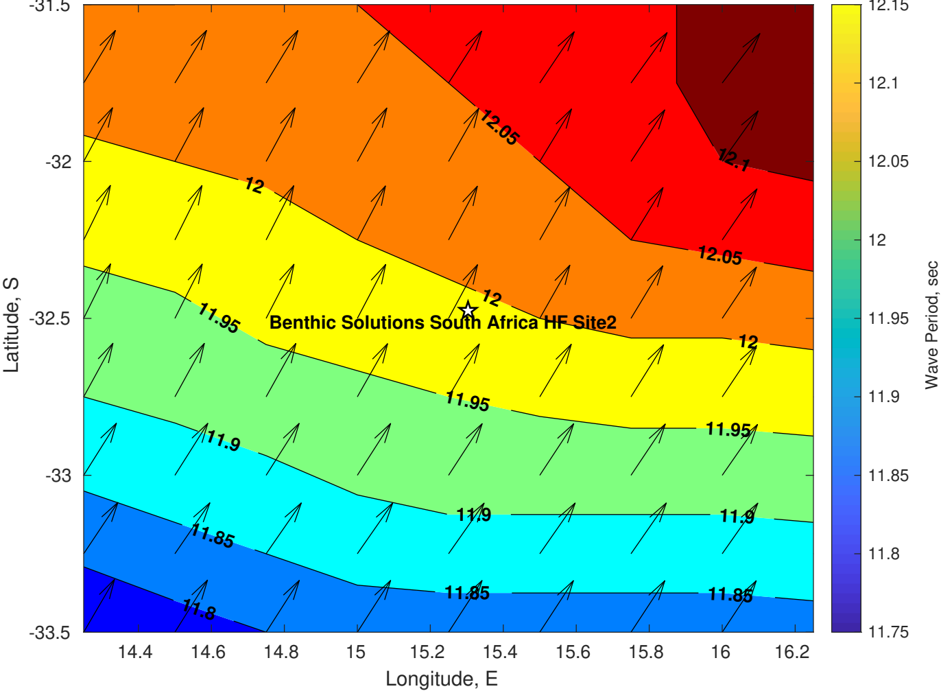
Wave Period (sec) for Benthic Solutions South Africa HF Site2 at 11-May-2025 09:00:00
