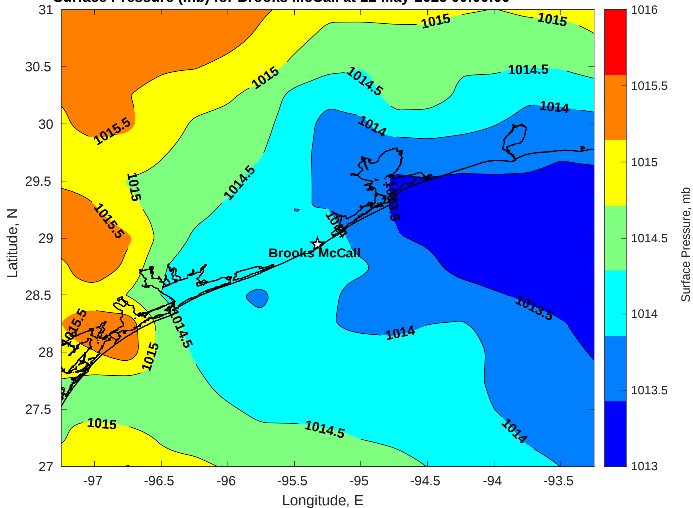
Surface Pressure (mb) for Brooks McCall at 11-May-2025 00:00:00
