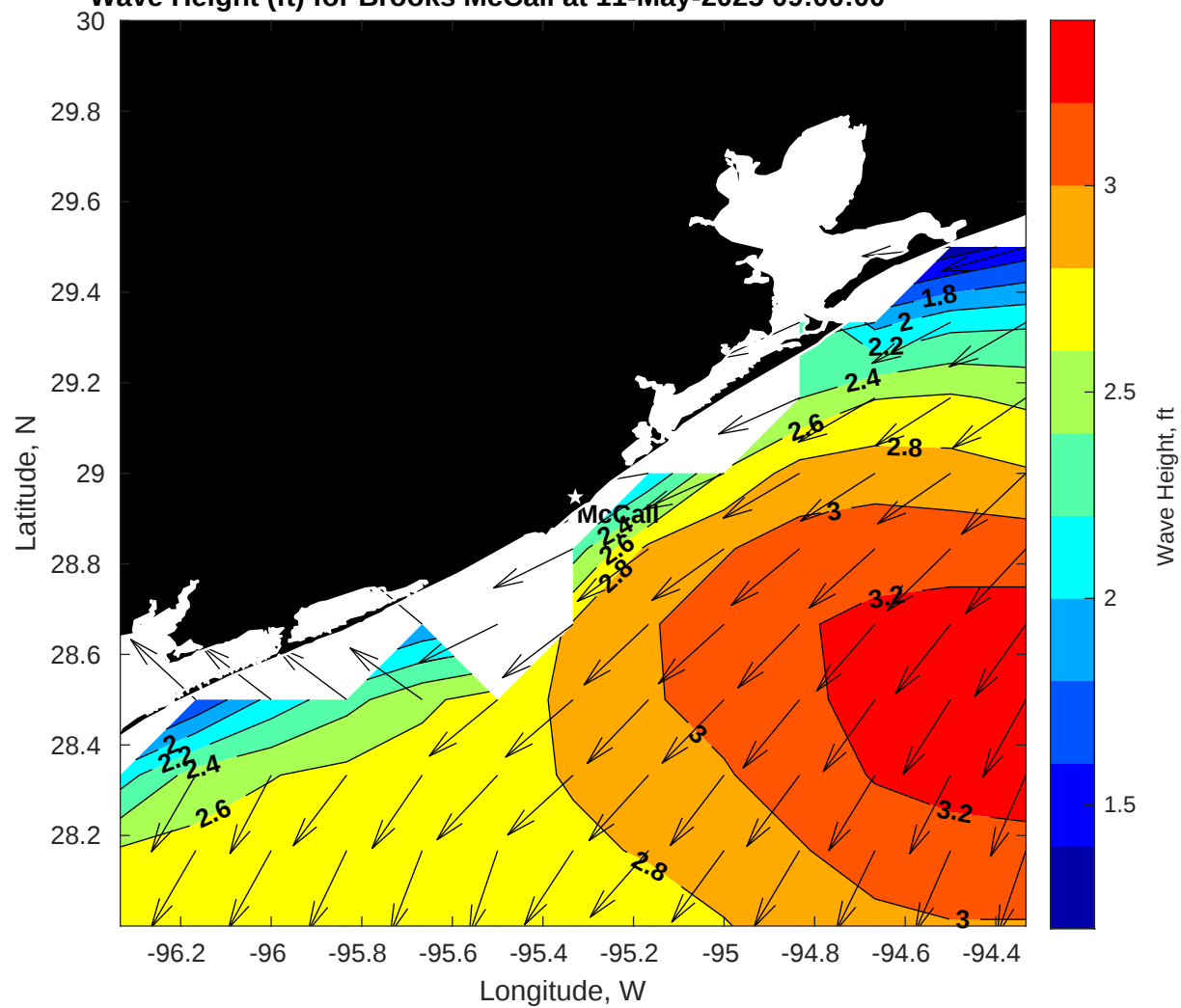
Wave Height (ft) for Brooks McCall at 11-May-2025 09:00:00
