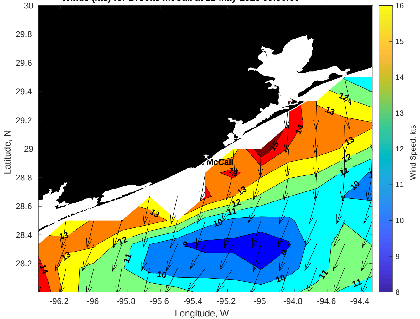
Winds (kts) for Brooks McCall at 11-May-2025 09:00:00
