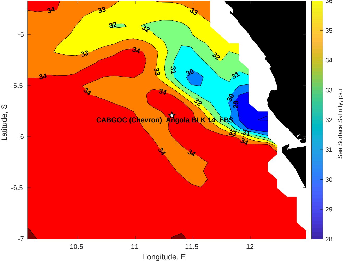
Surface Salinity for CABGOC (Chevron) Angola BLK 14 EBS at 10-May-2025 00:00:00
