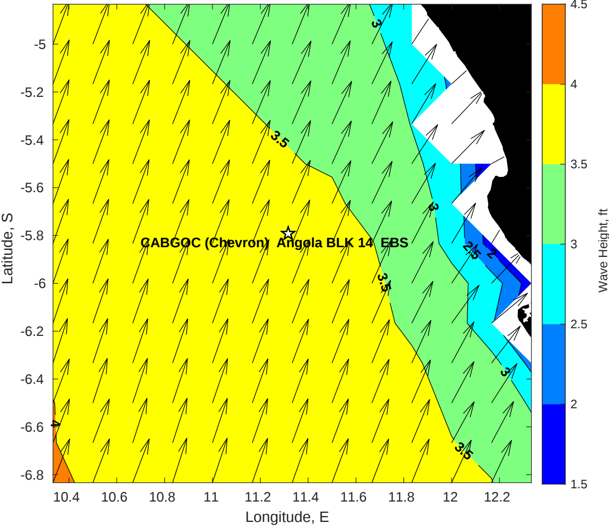
Wave Height (ft) for CABGOC (Chevron) Angola BLK 14 EBS at 11-May-2025 09:00:00
