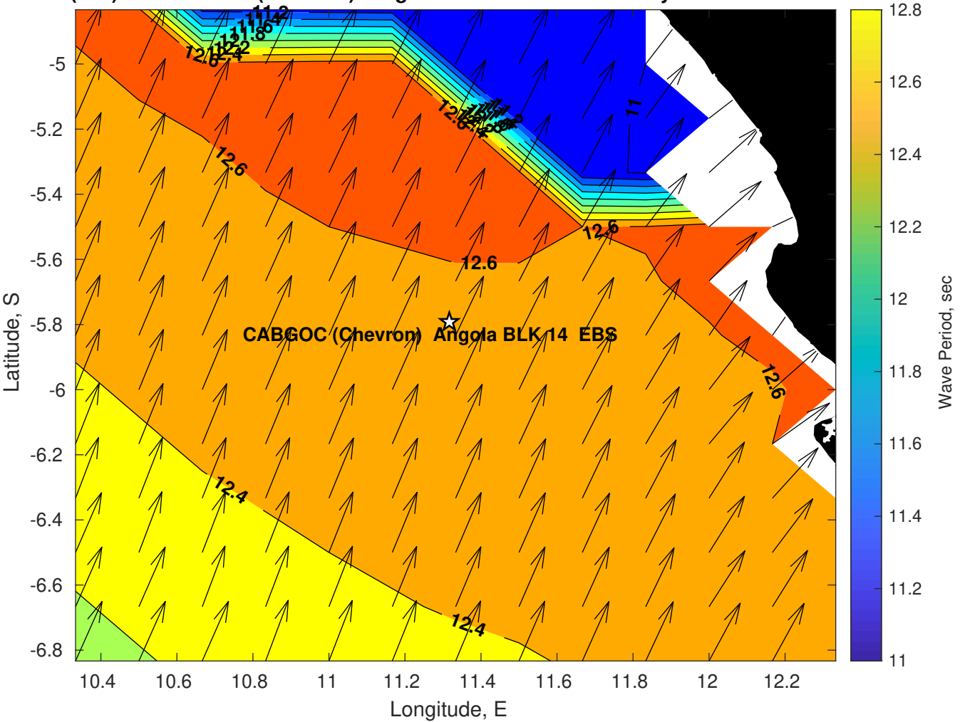
Wave Period (sec) for CABGOC (Chevron) Angola BLK 14 EBS at 11-May-2025 09:00:00
