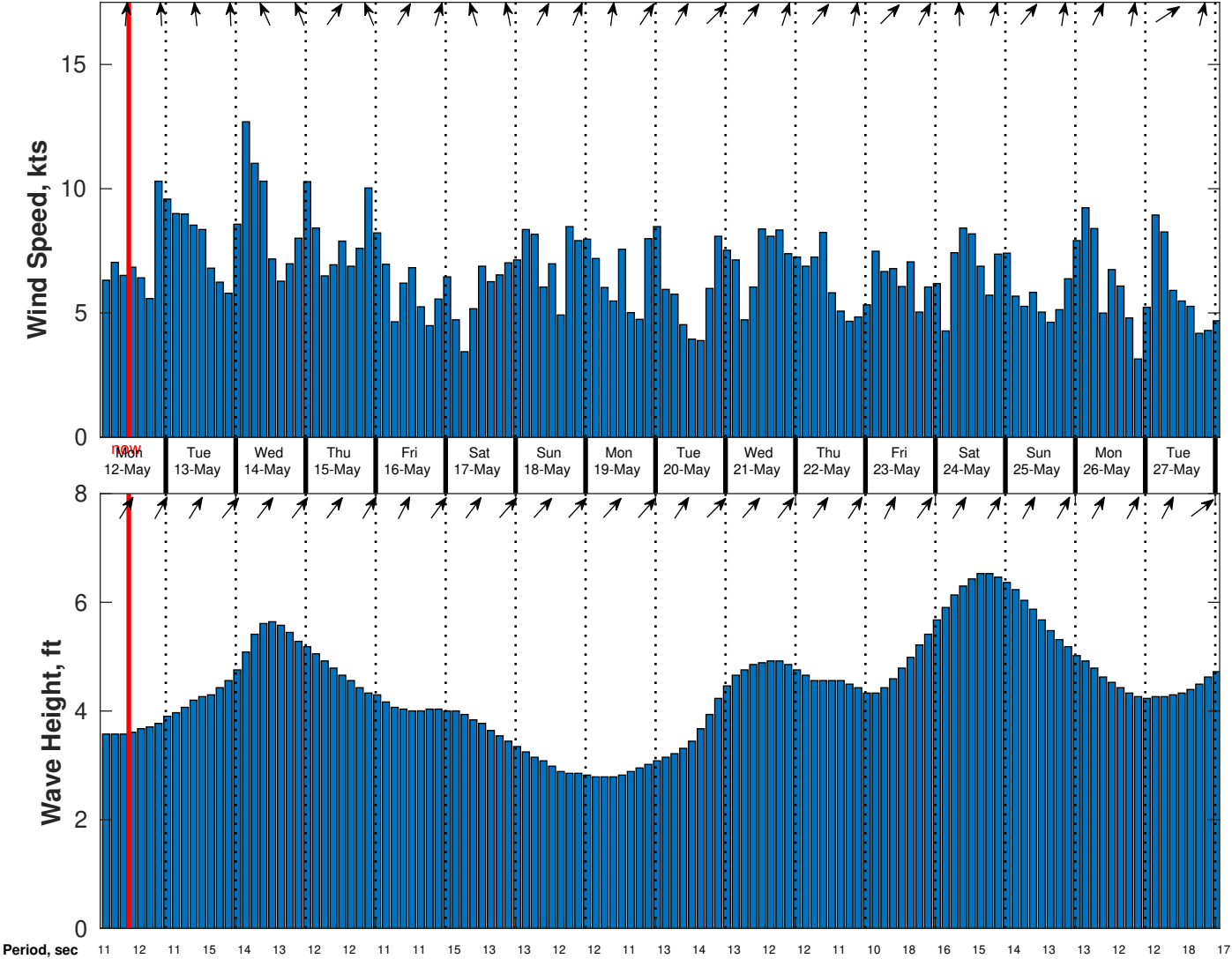
Wind & Wave Forecast for CABGOC (Chevron) Angola BLK 14 EBS from 11-May-2025 02:00:00 to 27-May-2025 02:00:00
