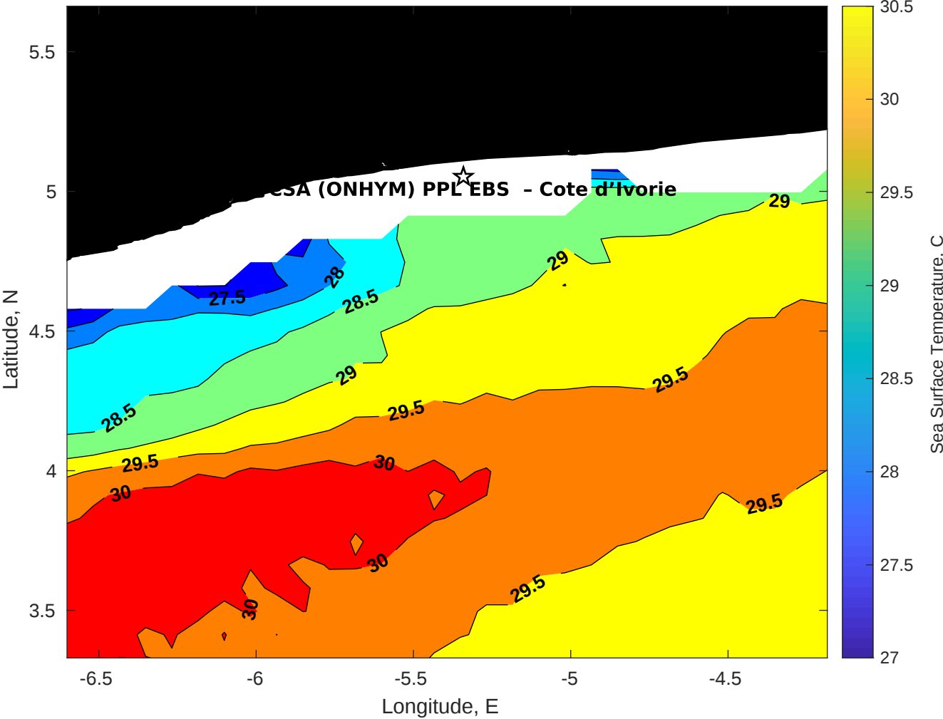
SST for CSA (ONHYM) PPL EBS - Cote d'Ivoire at 10-May-2025 00:00:00
