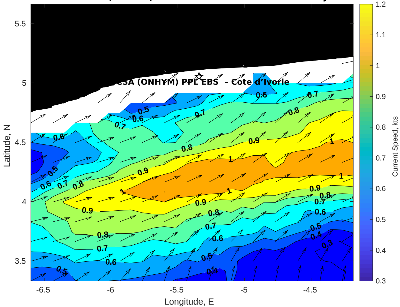
Surface Currents for CSA (ONHYM) PPL EBS - Cote d'Ivoire at 10-May-2025 00:00:00
