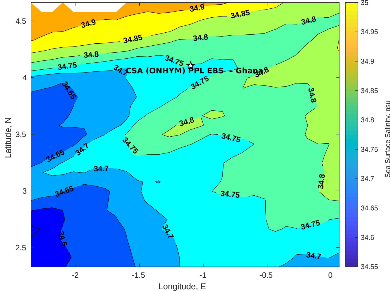
Surface Salinity for CSA (ONHYM) PPL EBS - Ghana at 10-May-2025 00:00:00
