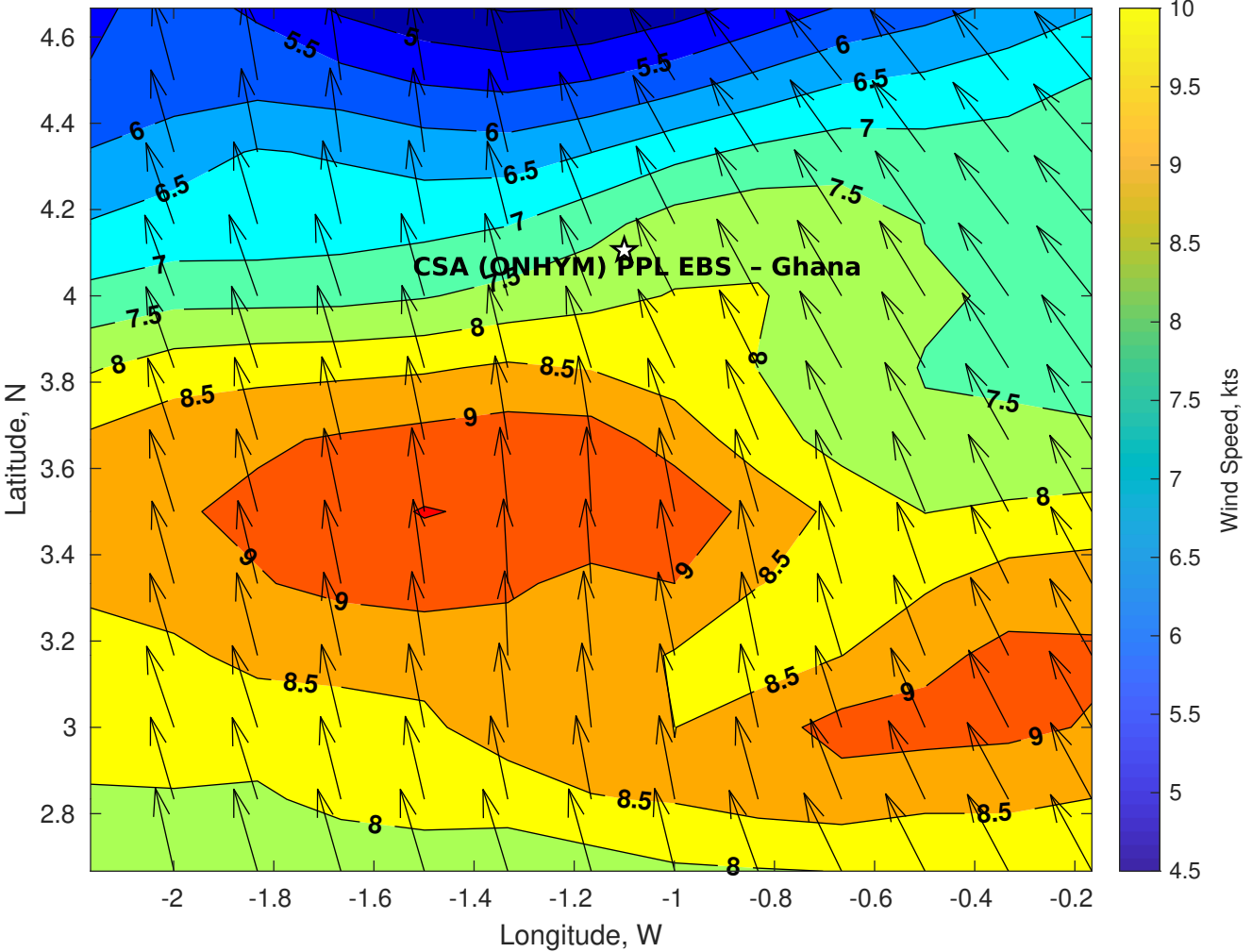
Winds (kts) for CSA (ONHYM) PPL EBS - Ghana at 11-May-2025 09:00:00
