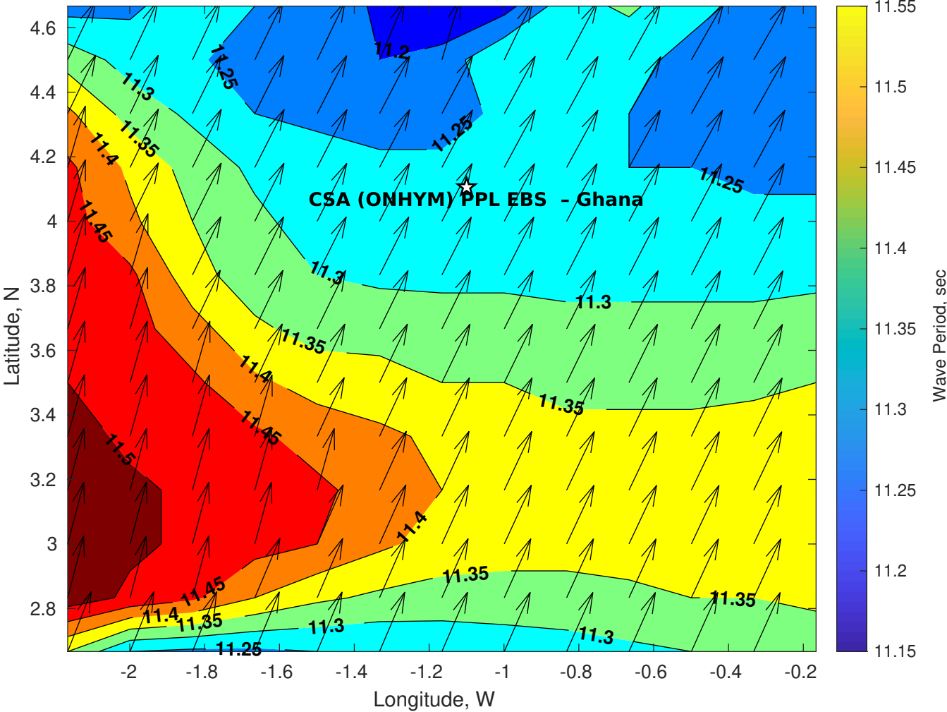
Wave Period (sec) for CSA (ONHYM) PPL EBS - Ghana at 11-May-2025 09:00:00
