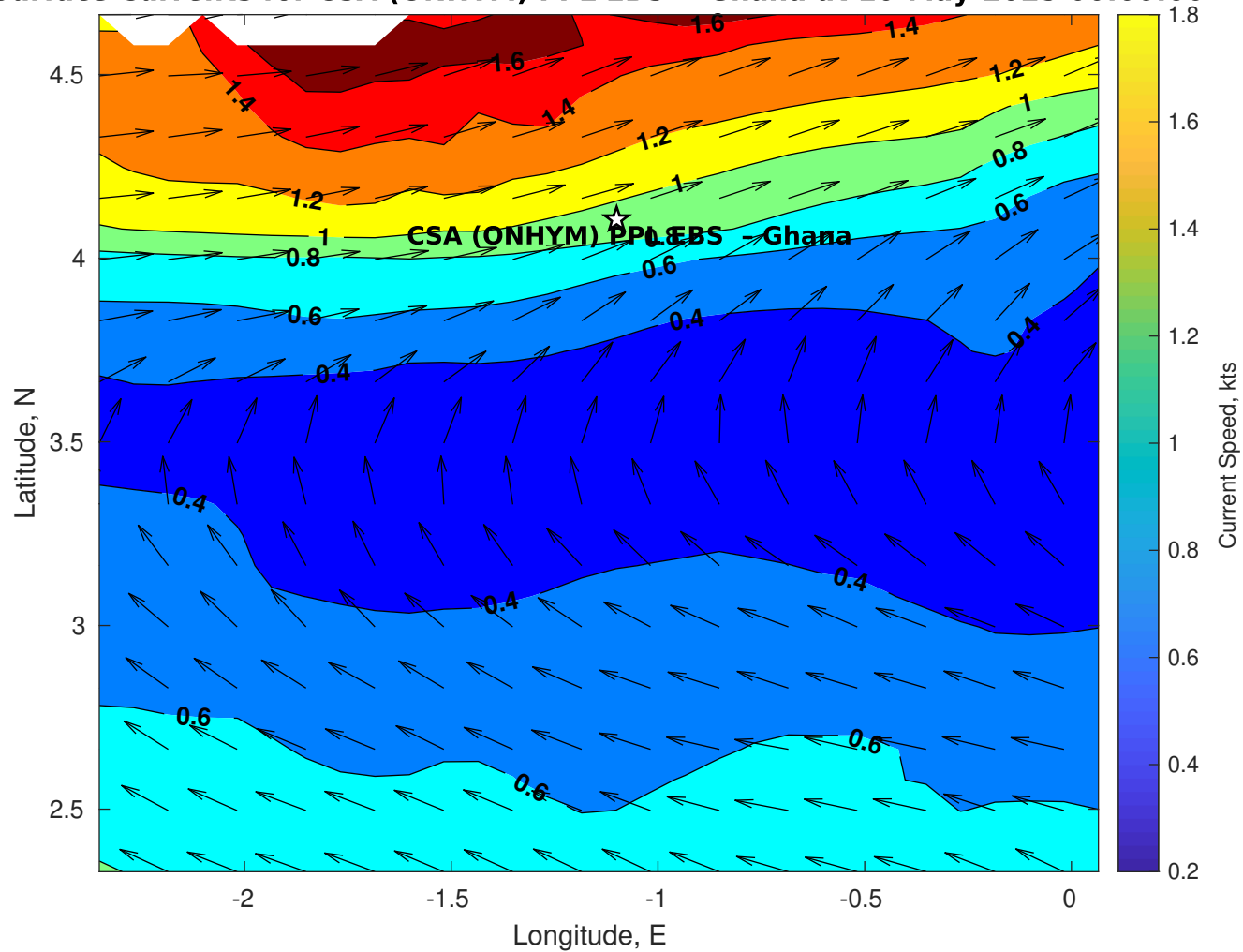
Surface Currents for CSA (ONHYM) PPL EBS - Ghana at 10-May-2025 00:00:00
