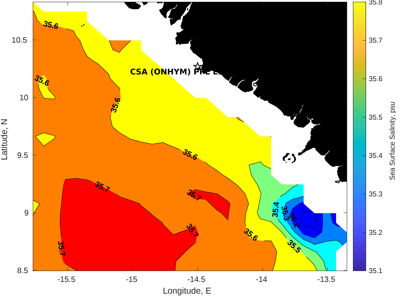
Surface Salinity for CSA (ONHYM) PPL EBS - Guinea at 10-May-2025 00:00:00
