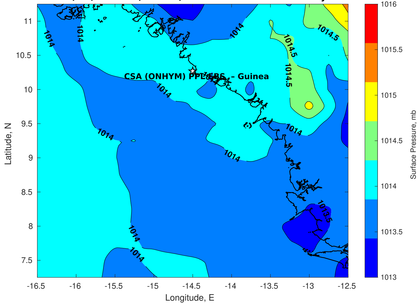
Surface Pressure (mb) for CSA (ONHYM) PPL EBS - Guinea at 11-May-2025 00:00:00
