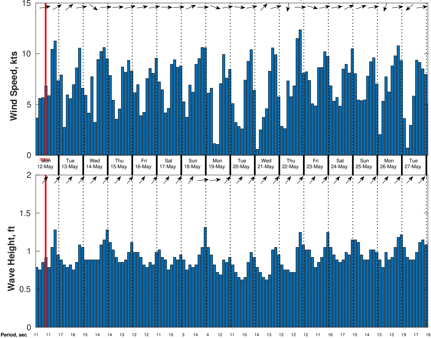
Wind & Wave Forecast for CSA (ONHYM) PPL EBS - Guinea from 11-May-2025 01:00:00 to 27-May-2025 01:00:00
