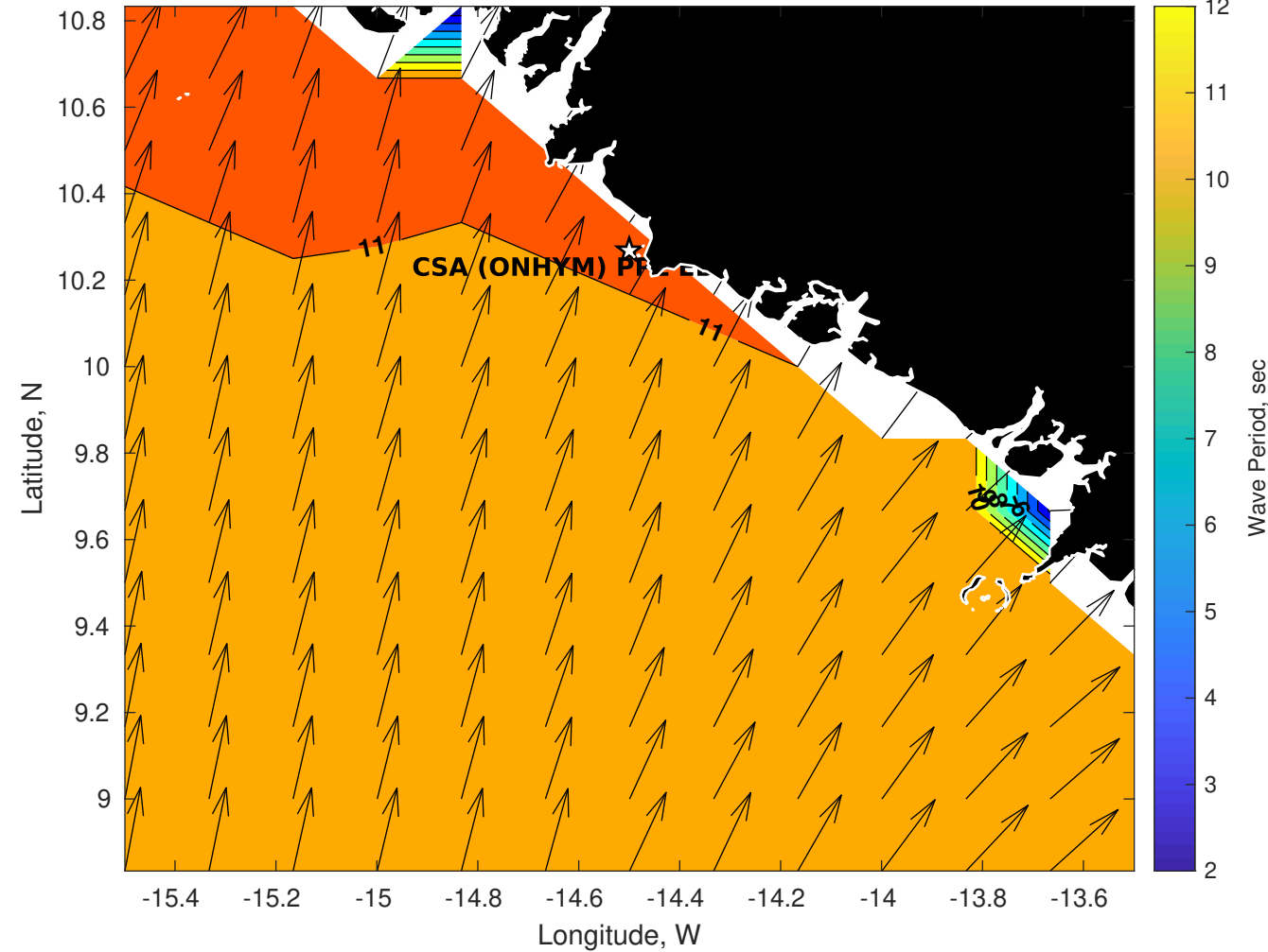
Wave Period (sec) for CSA (ONHYM) PPL EBS - Guinea at 11-May-2025 09:00:00
