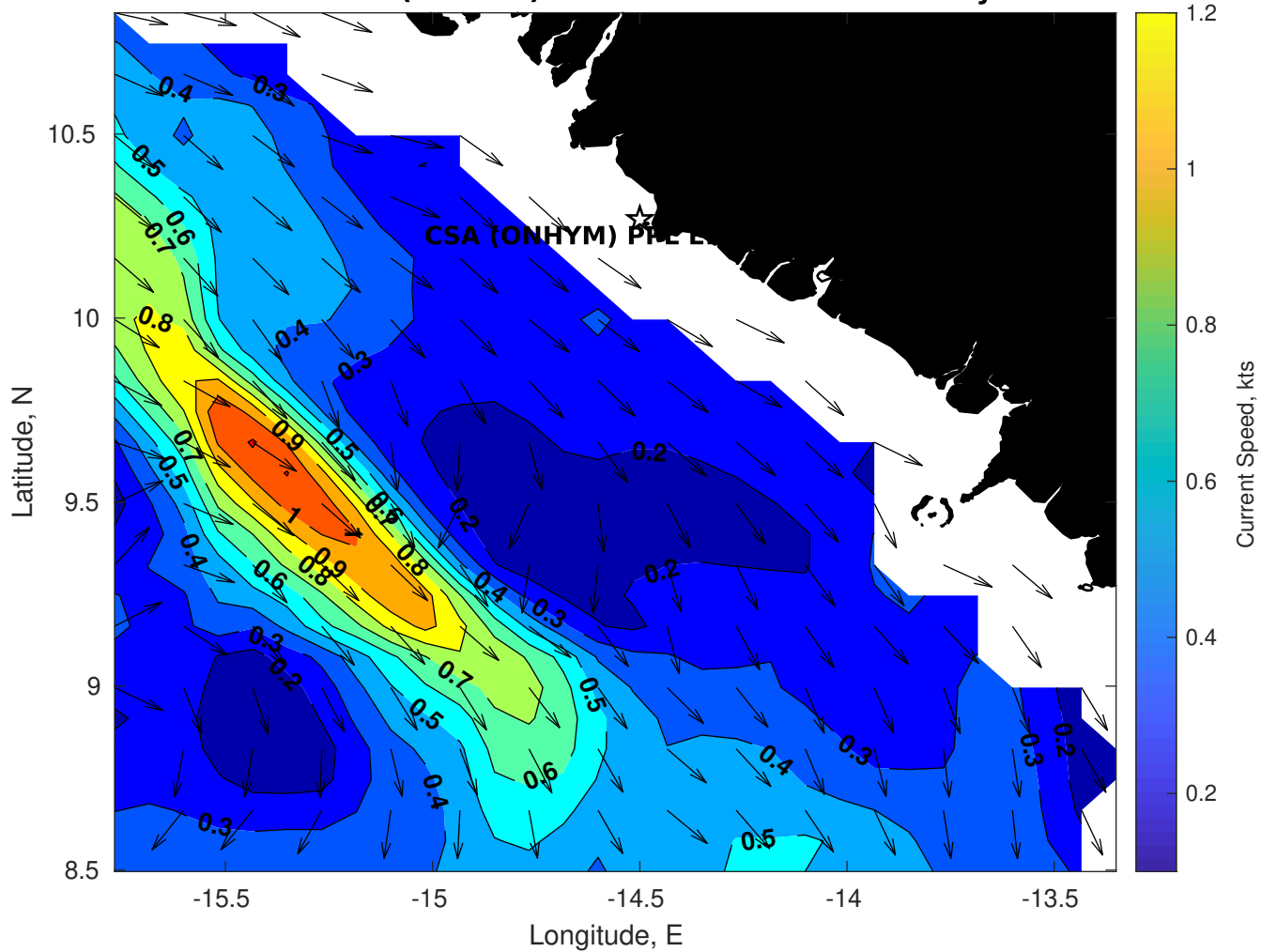
Surface Currents for CSA (ONHYM) PPL EBS - Guinea at 10-May-2025 00:00:00
