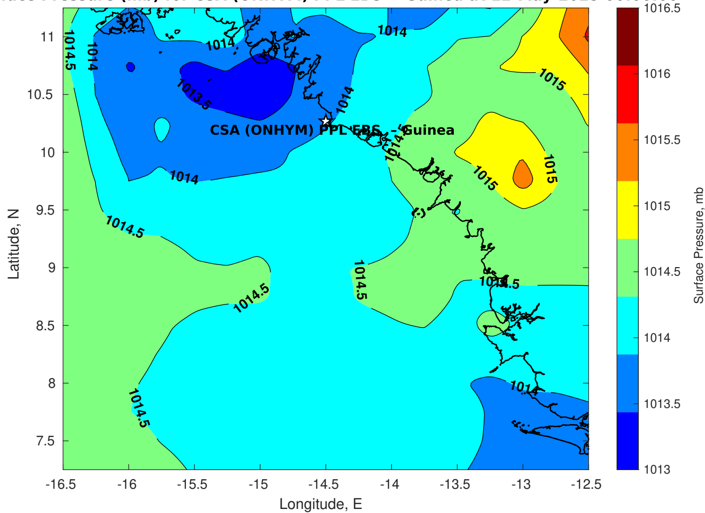
Surface Pressure (mb) for CSA (ONHYM) PPL EBS - Guinea at 12-May-2025 00:00:00
