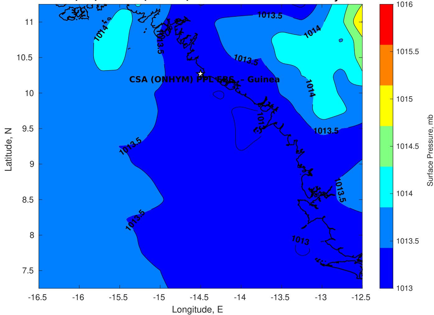
Surface Pressure (mb) for CSA (ONHYM) PPL EBS - Guinea at 13-May-2025 00:00:00
