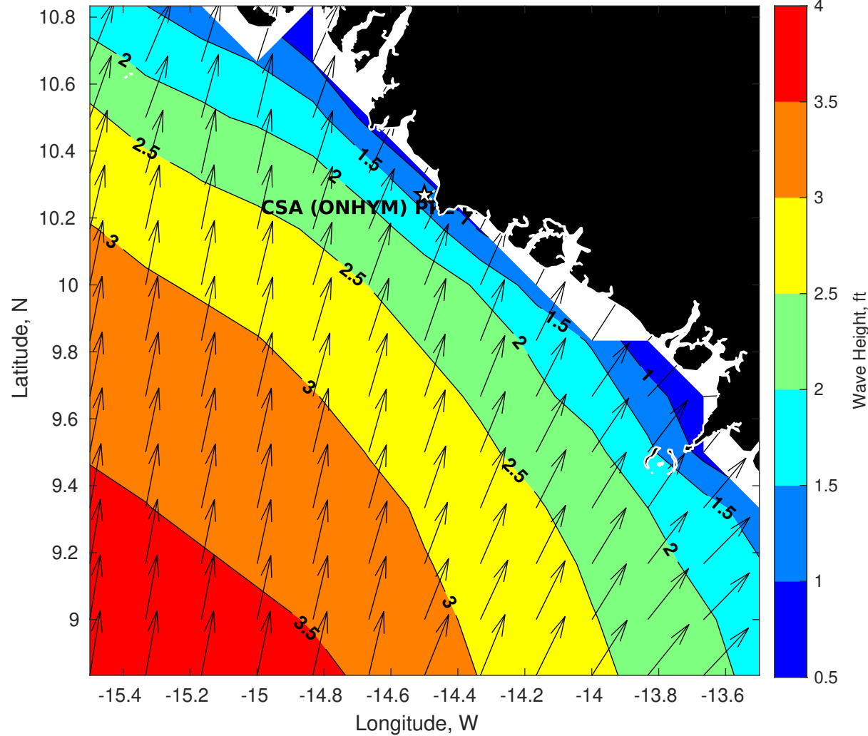
Wave Height (ft) for CSA (ONHYM) PPL EBS - Guinea at 11-May-2025 09:00:00
