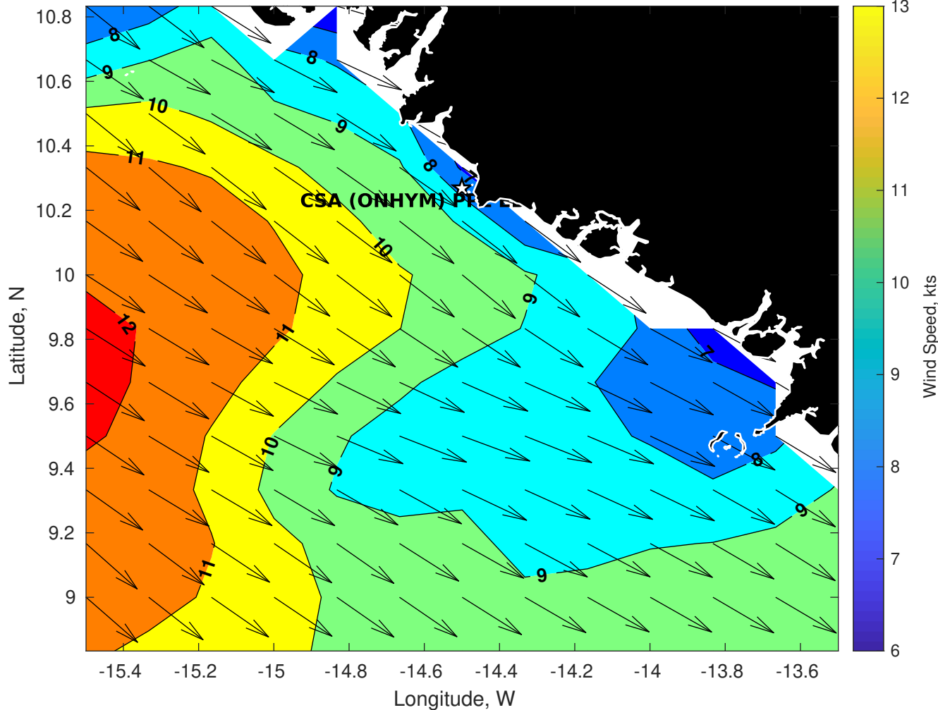
Winds (kts) for CSA (ONHYM) PPL EBS - Guinea at 11-May-2025 09:00:00
