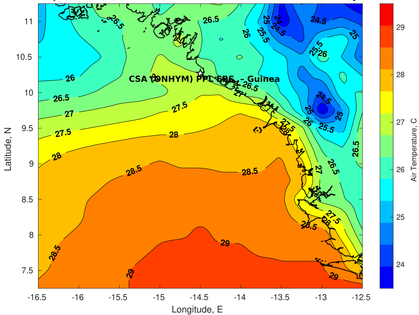
Air Temperature (C) for CSA (ONHYM) PPL EBS - Guinea at 11-May-2025
