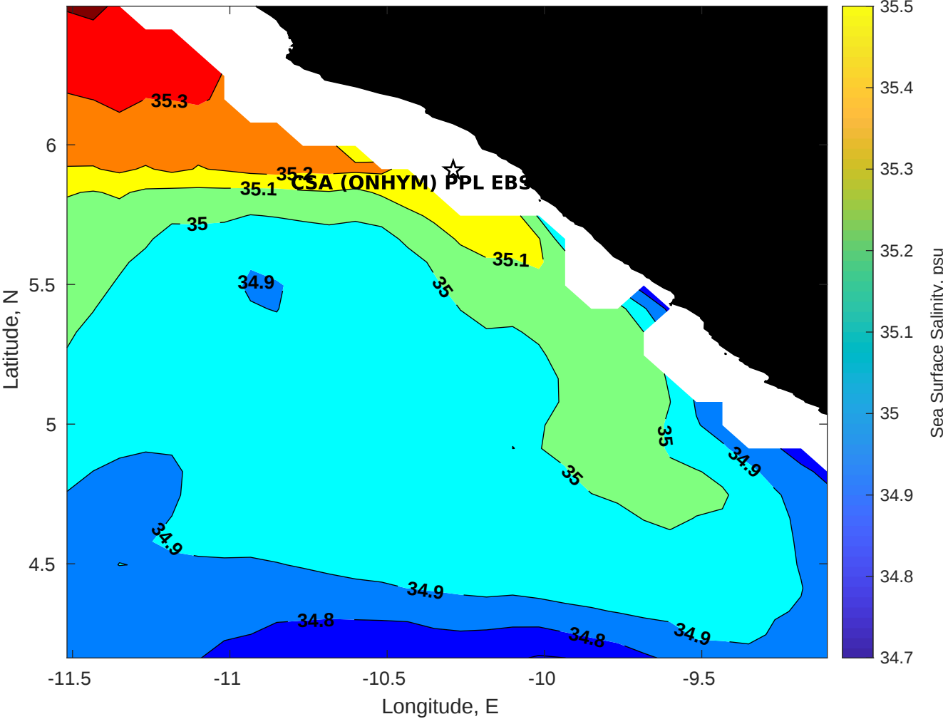
Surface Salinity for CSA (ONHYM) PPL EBS - Liberia at 10-May-2025 00:00:00
