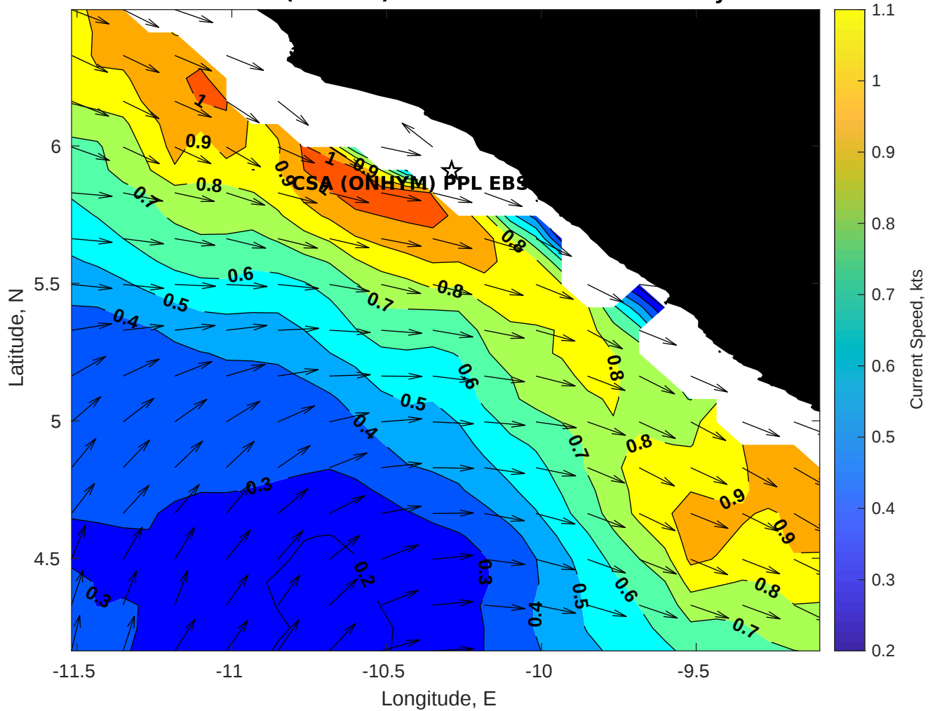
Surface Currents for CSA (ONHYM) PPL EBS - Liberia at 10-May-2025 00:00:00
