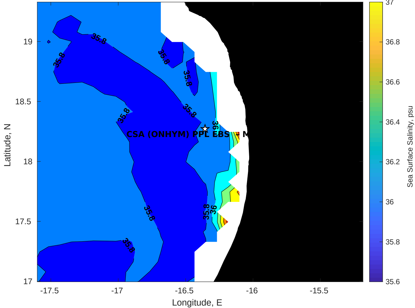
Surface Salinity for CSA (ONHYM) PPL EBS - Mauritania at 10-May-2025 00:00:00
