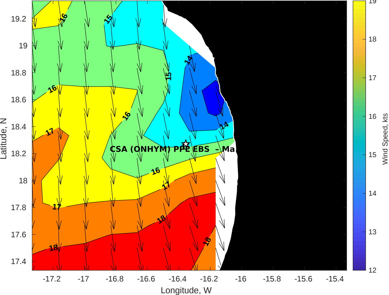
Winds (kts) for CSA (ONHYM) PPL EBS - Mauritania at 11-May-2025 09:00:00
