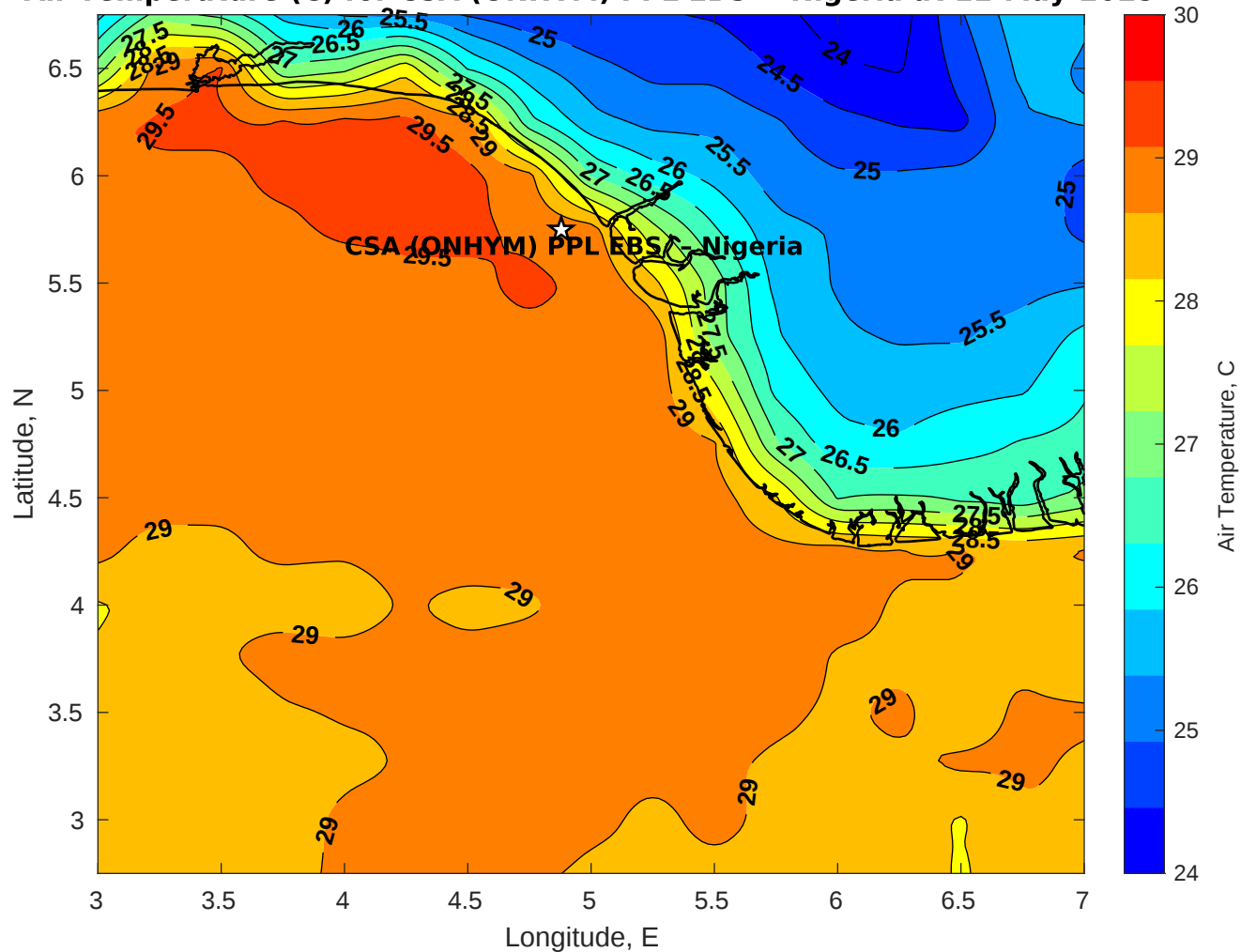
Air Temperature (C) for CSA (ONHYM) PPL EBS - Nigeria at 11-May-2025
