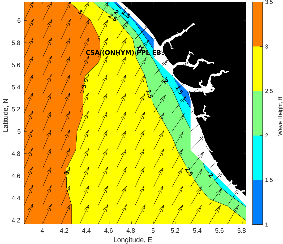
Wave Height (ft) for CSA (ONHYM) PPL EBS - Nigeria at 11-May-2025 09:00:00
