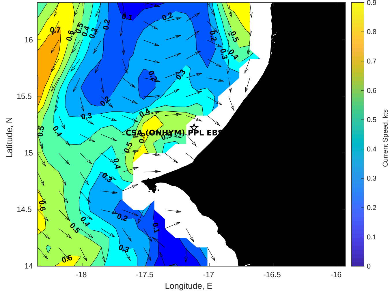
Surface Currents for CSA (ONHYM) PPL EBS - Senegal at 10-May-2025 00:00:00
