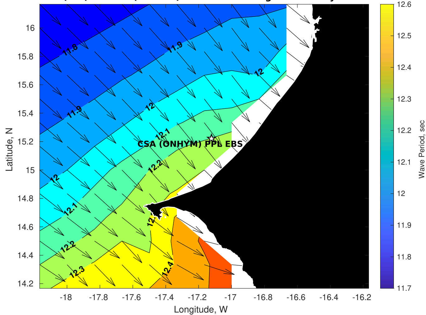
Wave Period (sec) for CSA (ONHYM) PPL EBS - Senegal at 11-May-2025 09:00:00
