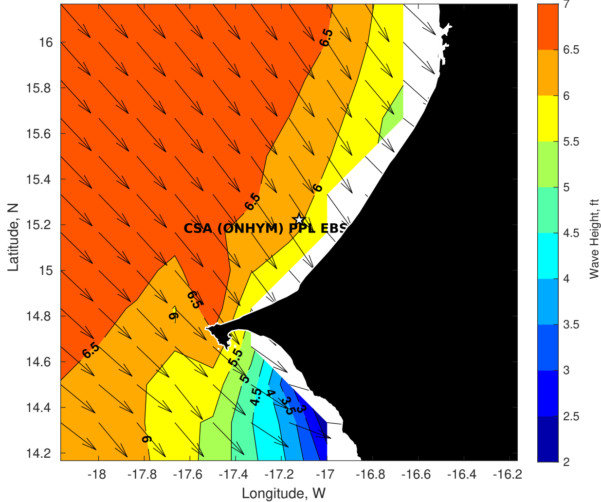
Wave Height (ft) for CSA (ONHYM) PPL EBS - Senegal at 11-May-2025 09:00:00
