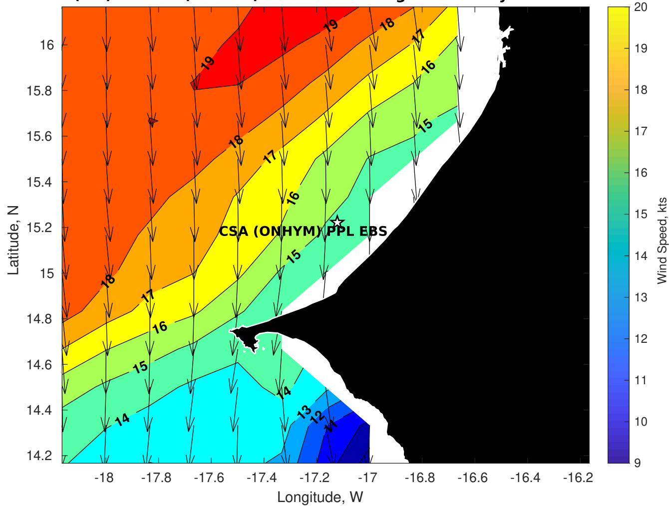
Winds (kts) for CSA (ONHYM) PPL EBS - Senegal at 11-May-2025 09:00:00
