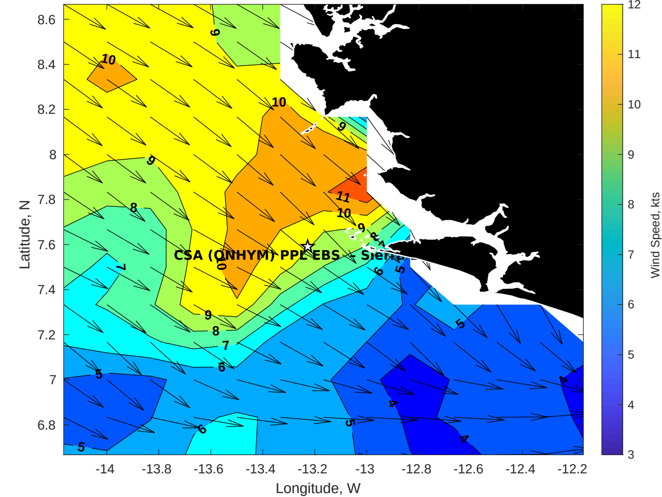
Winds (kts) for CSA (ONHYM) PPL EBS - Sierra Leone at 11-May-2025 09:00:00
