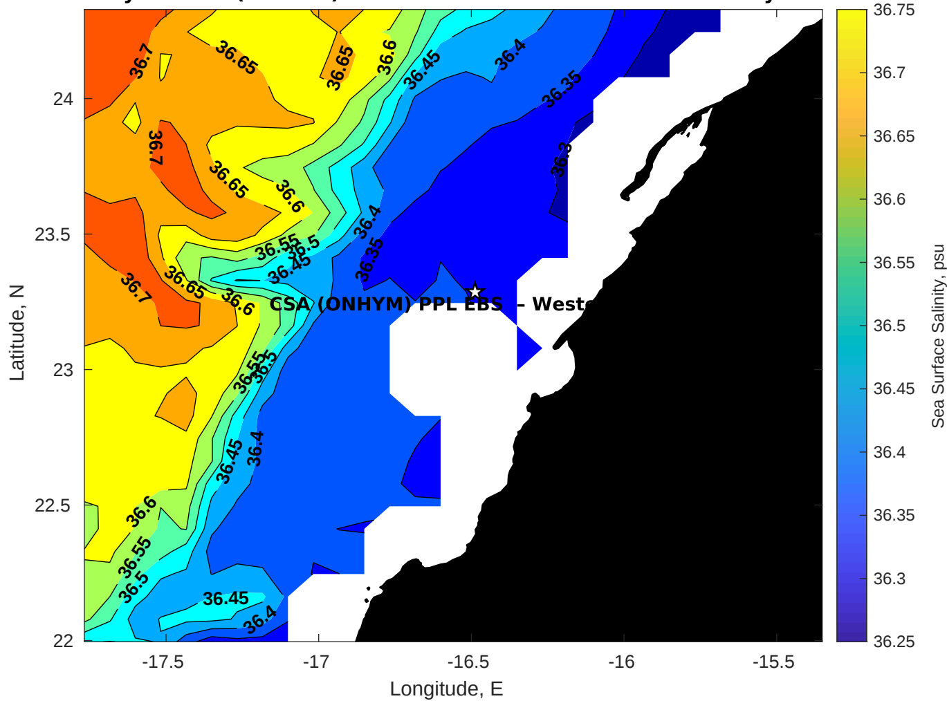
Surface Salinity for CSA (ONHYM) PPL EBS - Western Sahara at 10-May-2025 00:00:00
