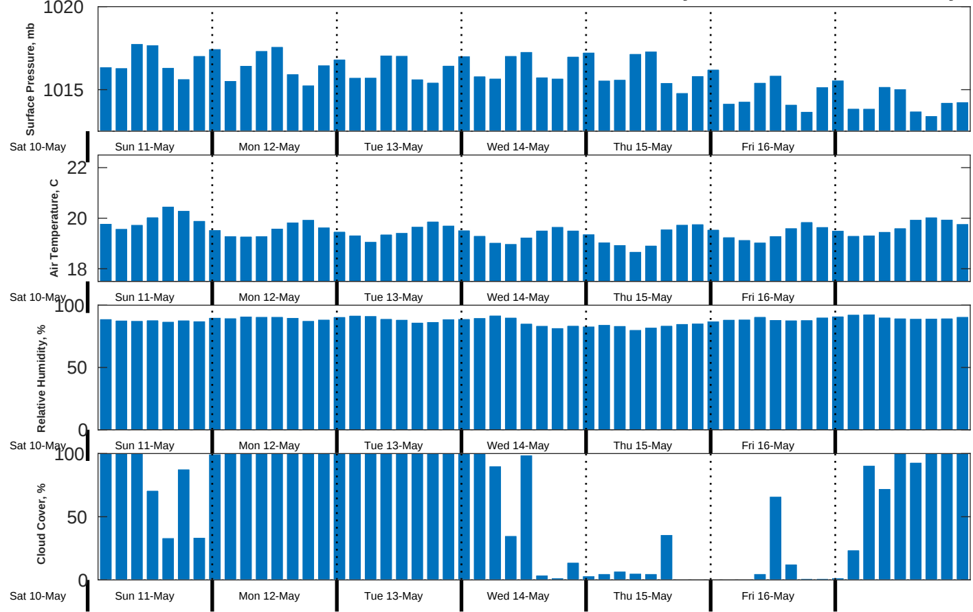
Met Forecast for CSA (ONHYM) PPL EBS - Western Sahara from 11-May-2025 00:00:00 to 18-May-2025 00:00:00
