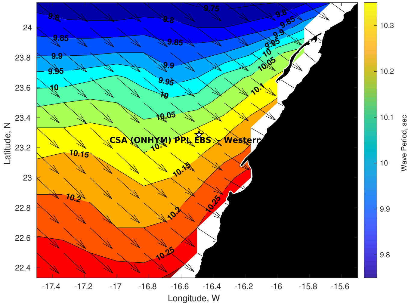
Wave Period (sec) for CSA (ONHYM) PPL EBS - Western Sahara at 11-May-2025 09:00:00
