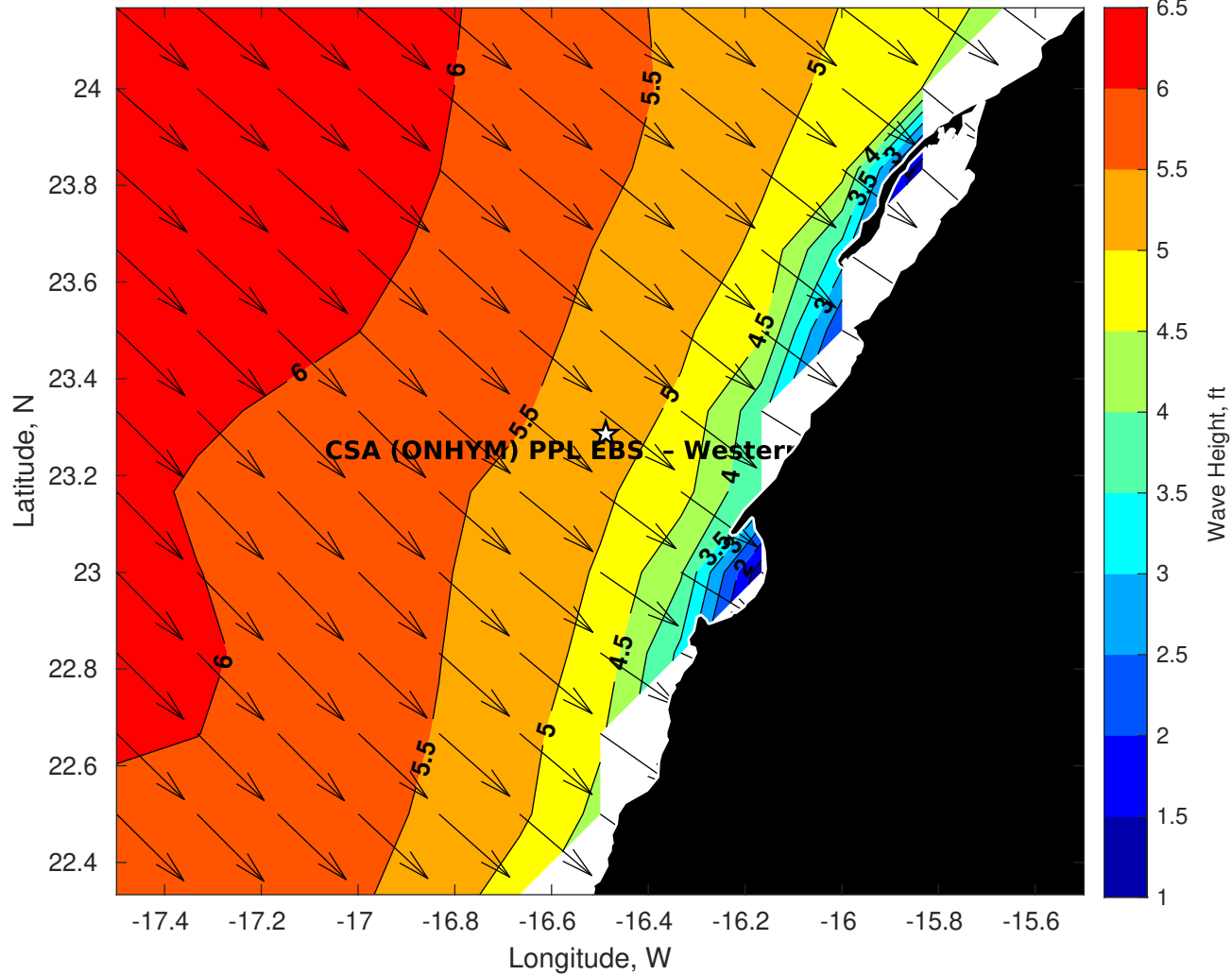
Wave Height (ft) for CSA (ONHYM) PPL EBS - Western Sahara at 11-May-2025 09:00:00
