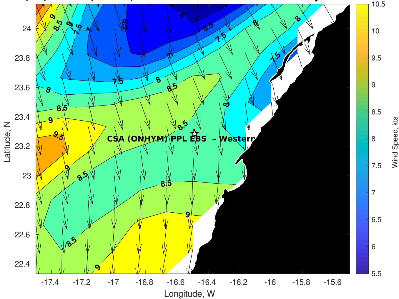
Winds (kts) for CSA (ONHYM) PPL EBS - Western Sahara at 11-May-2025 09:00:00
