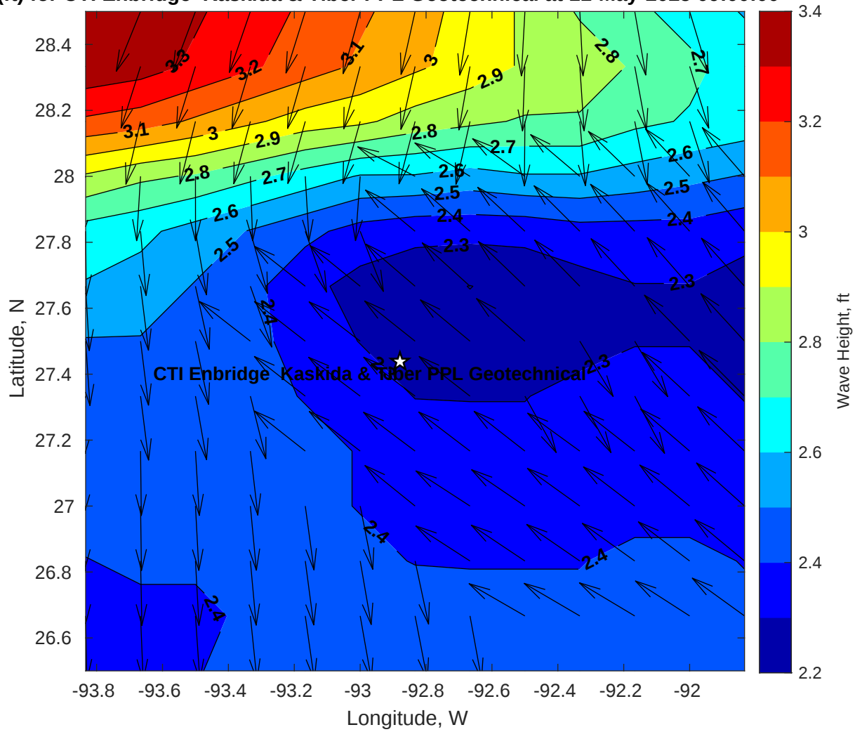
Wave Height (ft) for CTI Enbridge Kaskida & Tiber PPL Geotechnical at 11-May-2025 09:00:00
