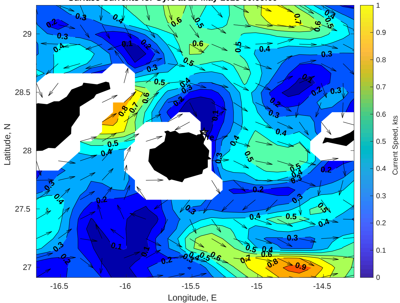
Surface Currents for Gyre at 10-May-2025 00:00:00
