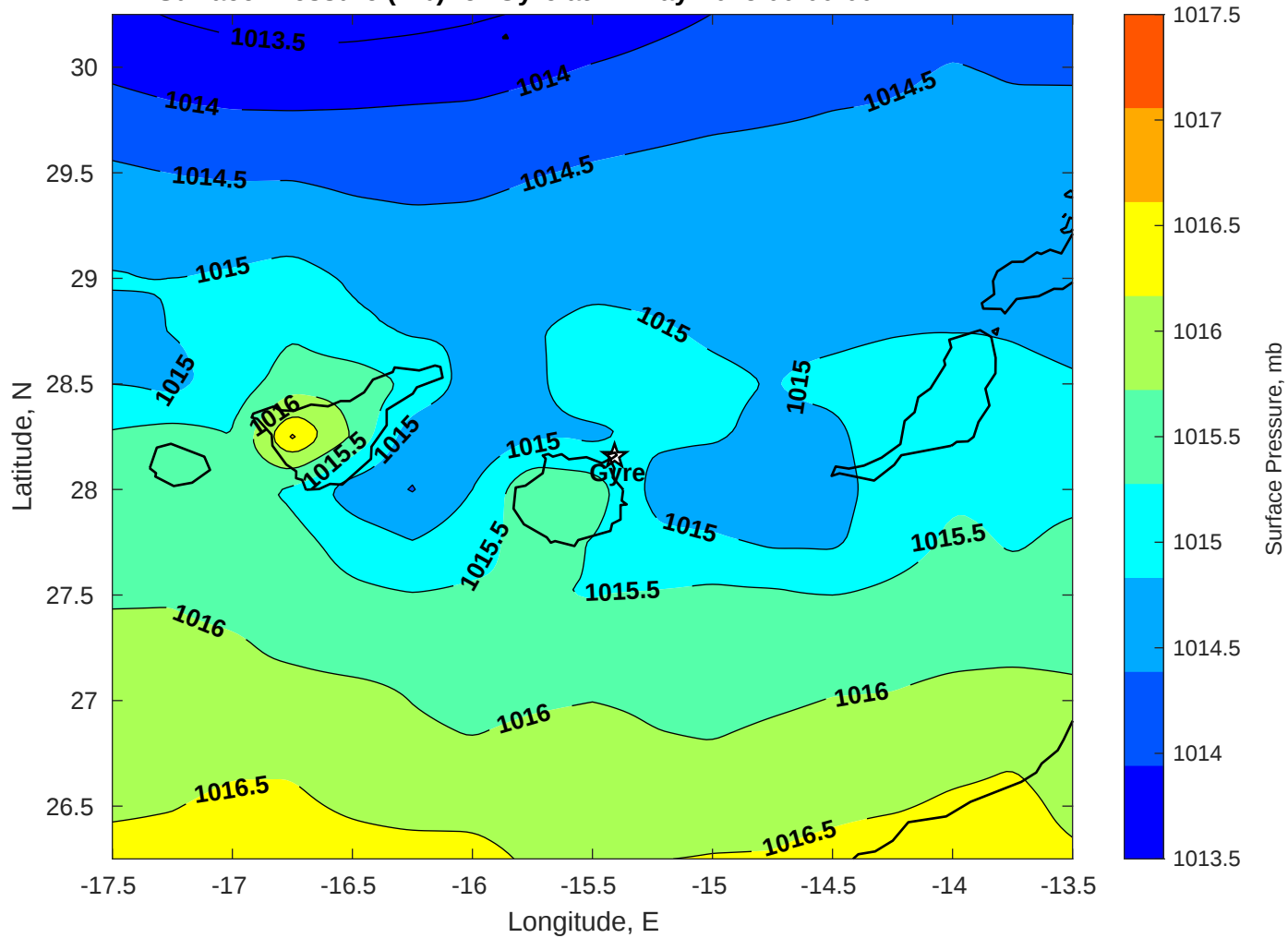
Surface Pressure (mb) for Gyre at 11-May-2025 00:00:00
