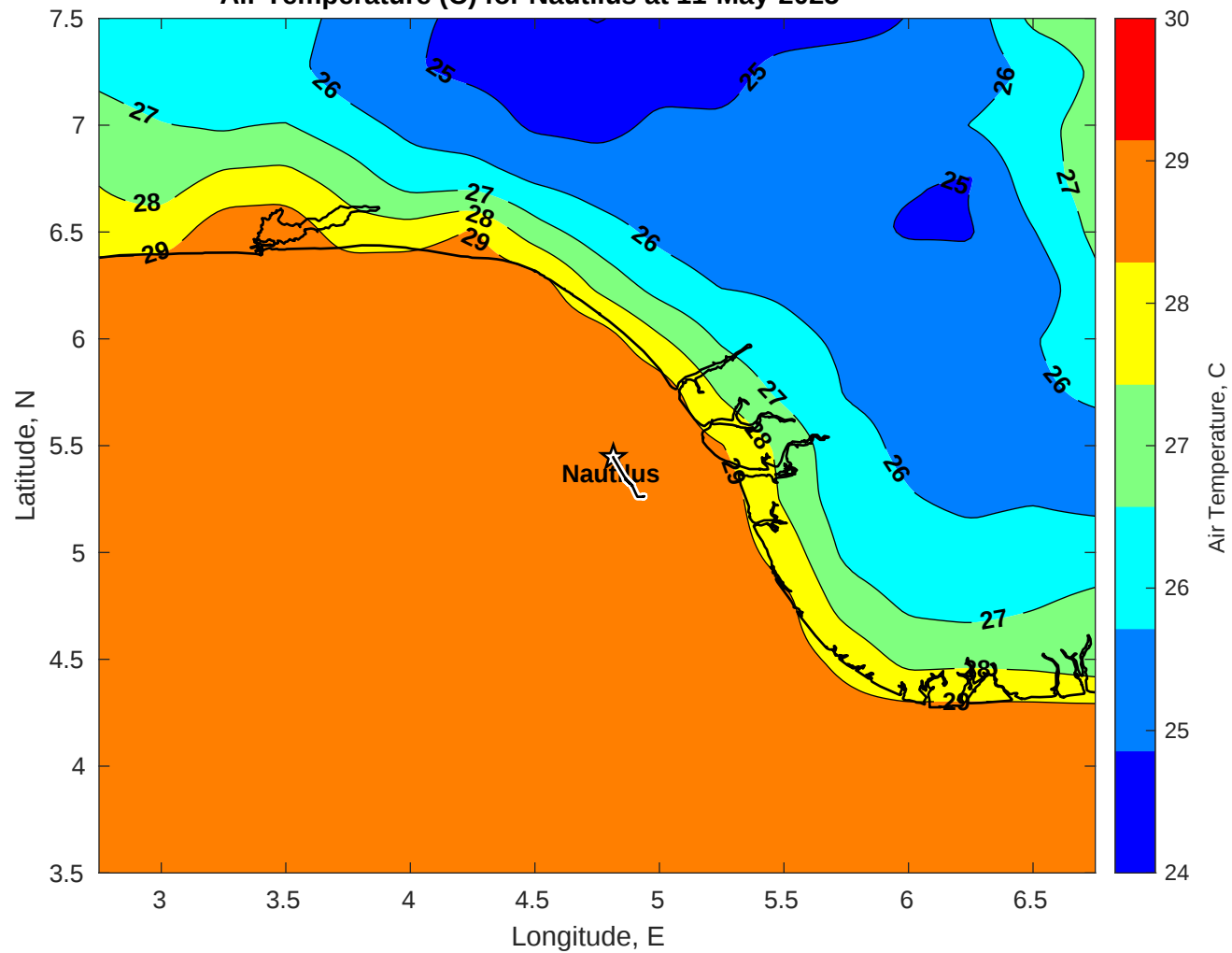
Air Temperature (C) for Nautilus at 11-May-2025
