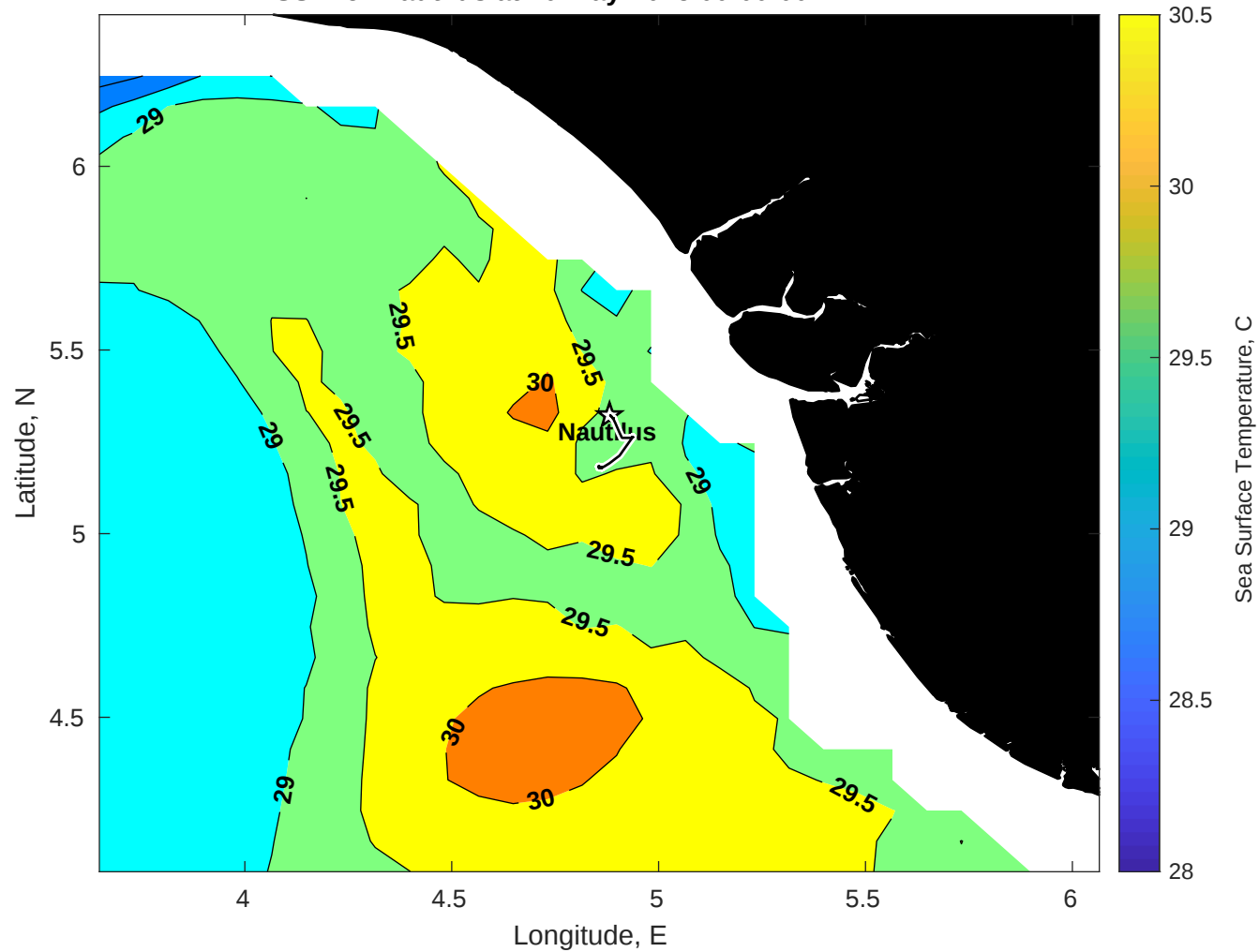
SST for Nautilus at 10-May-2025 00:00:00
