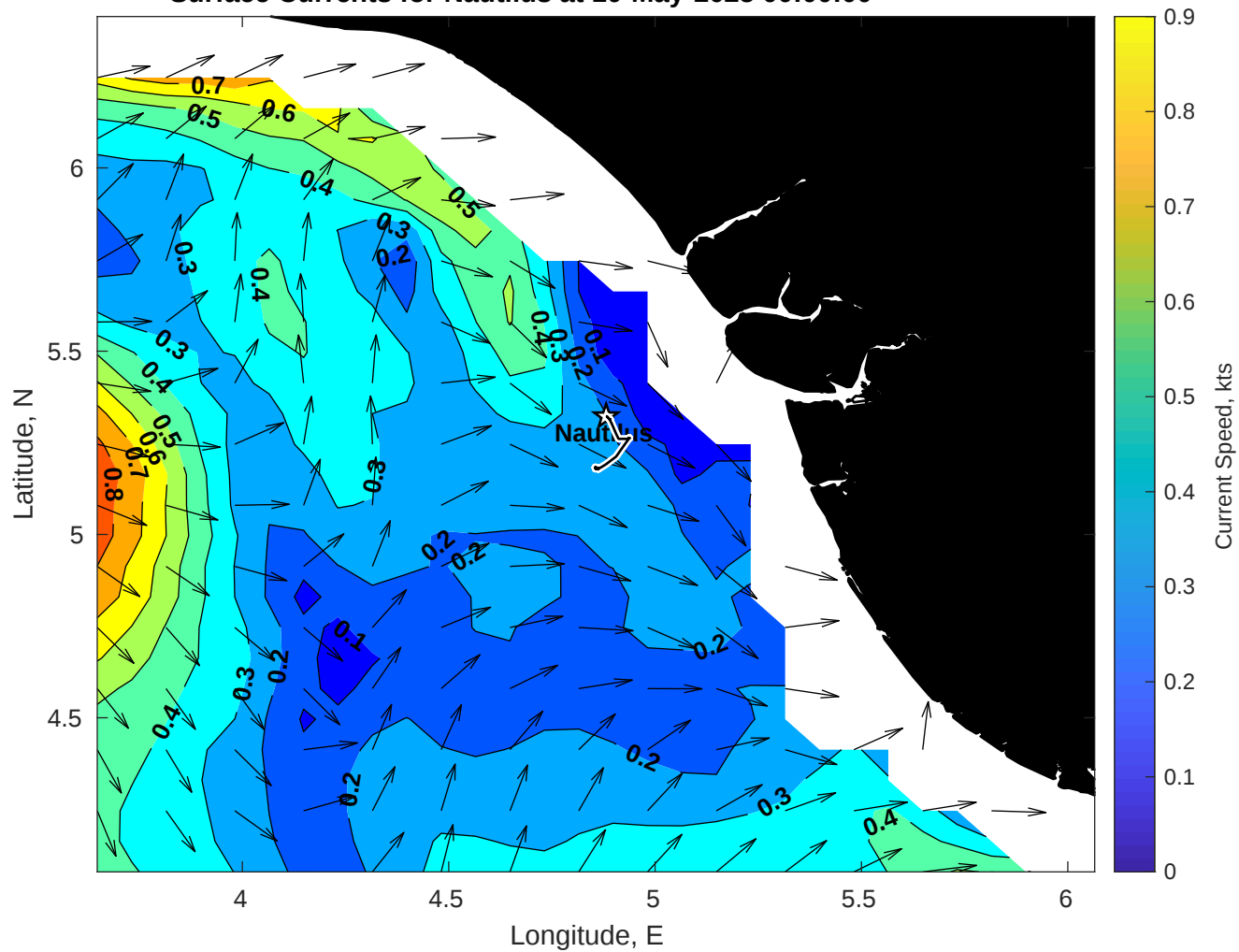
Surface Currents for Nautilus at 10-May-2025 00:00:00
