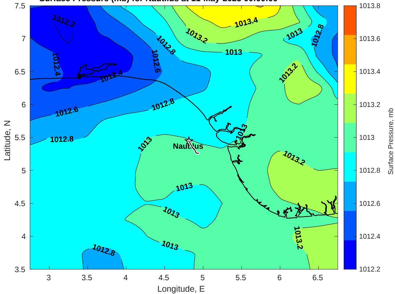
Surface Pressure (mb) for Nautilus at 11-May-2025 00:00:00
