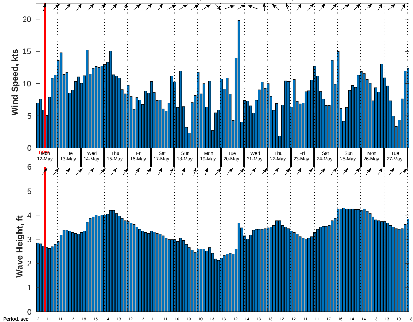
Wind & Wave Forecast for Nautilus from 11-May-2025 02:00:00 to 27-May-2025 02:00:00
