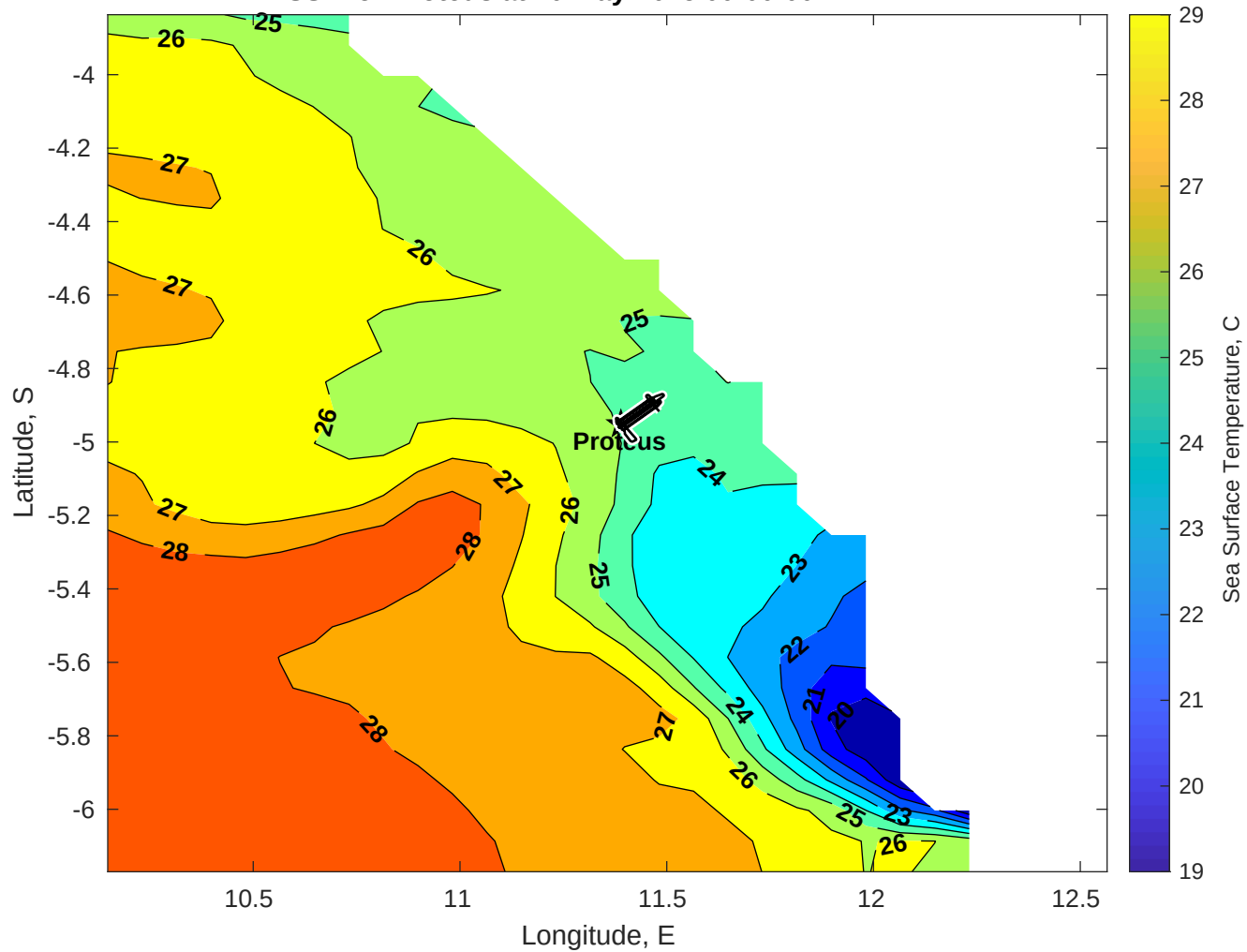
SST for Proteus at 10-May-2025 00:00:00
