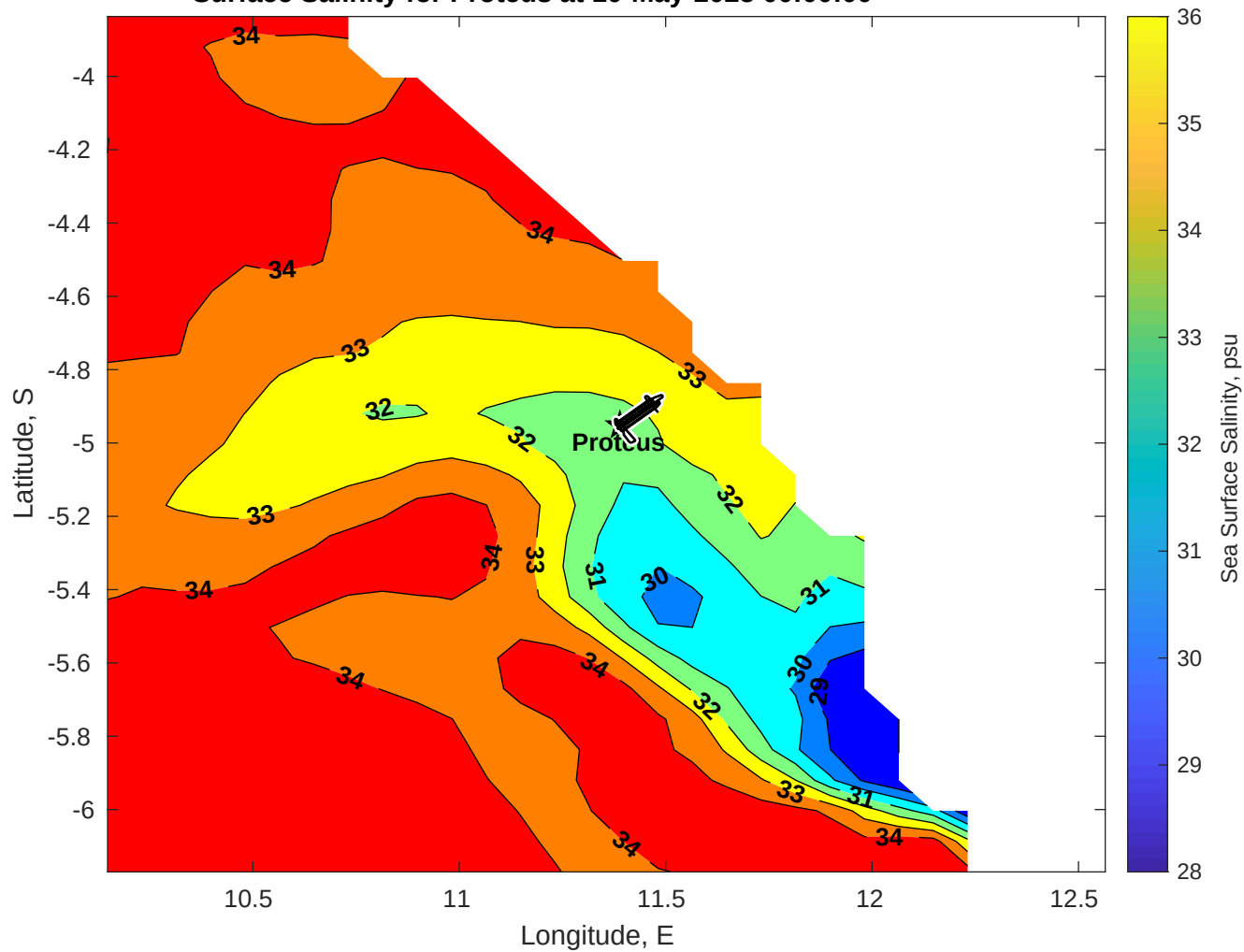
Surface Salinity for Proteus at 10-May-2025 00:00:00
