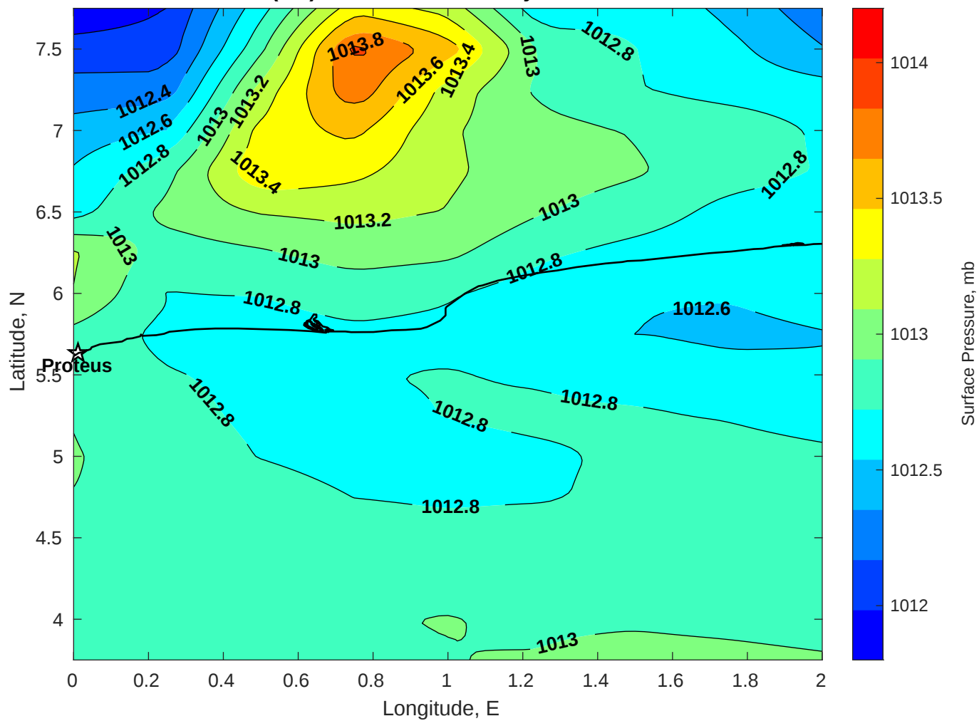
Surface Pressure (mb) for Proteus at 11-May-2025 00:00:00
