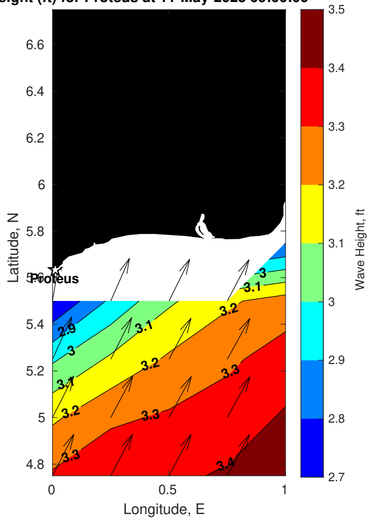
Wave Height (ft) for Proteus at 11-May-2025 09:00:00
