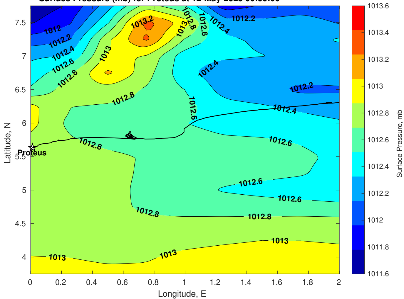
Surface Pressure (mb) for Proteus at 12-May-2025 00:00:00
