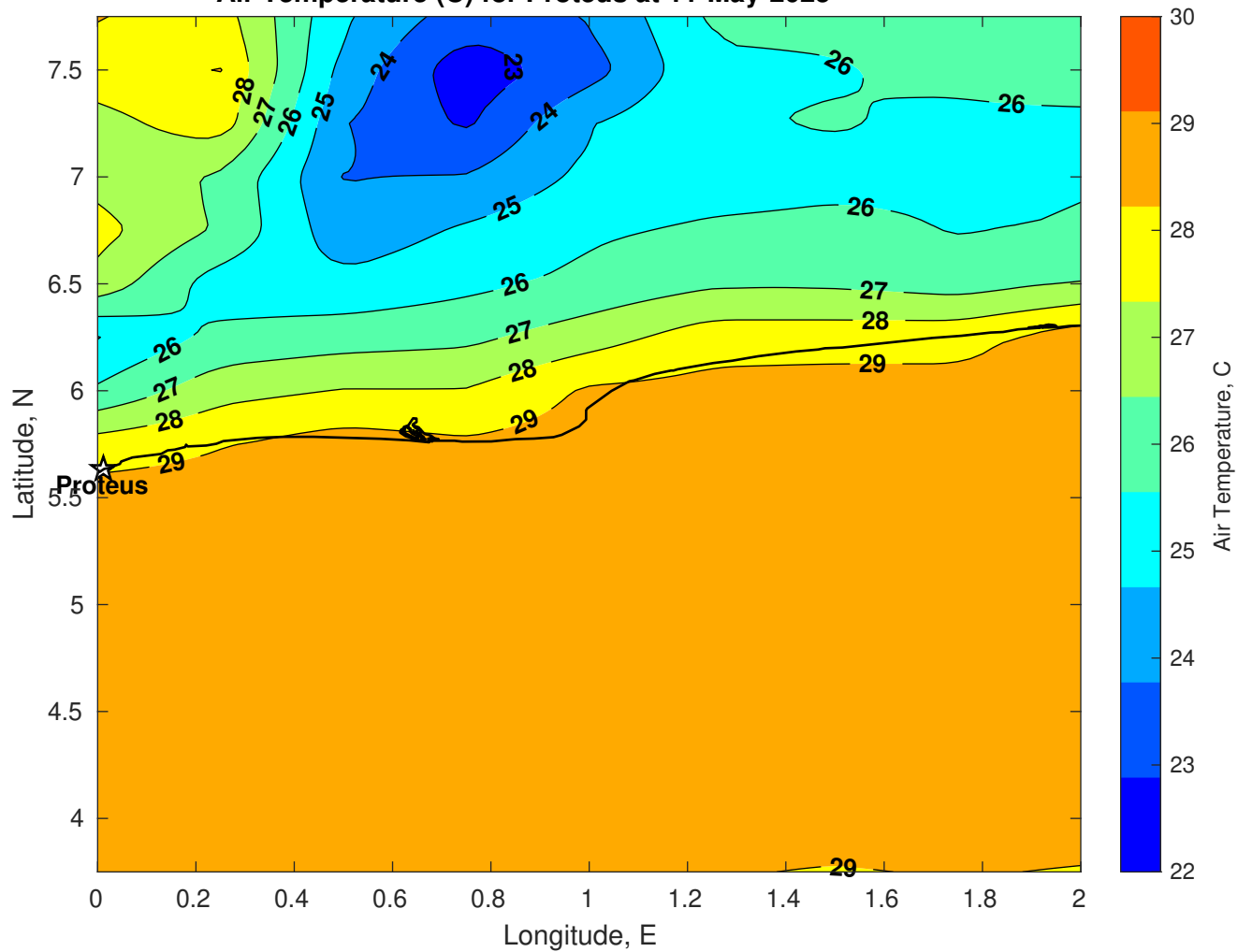
Air Temperature (C) for Proteus at 11-May-2025
