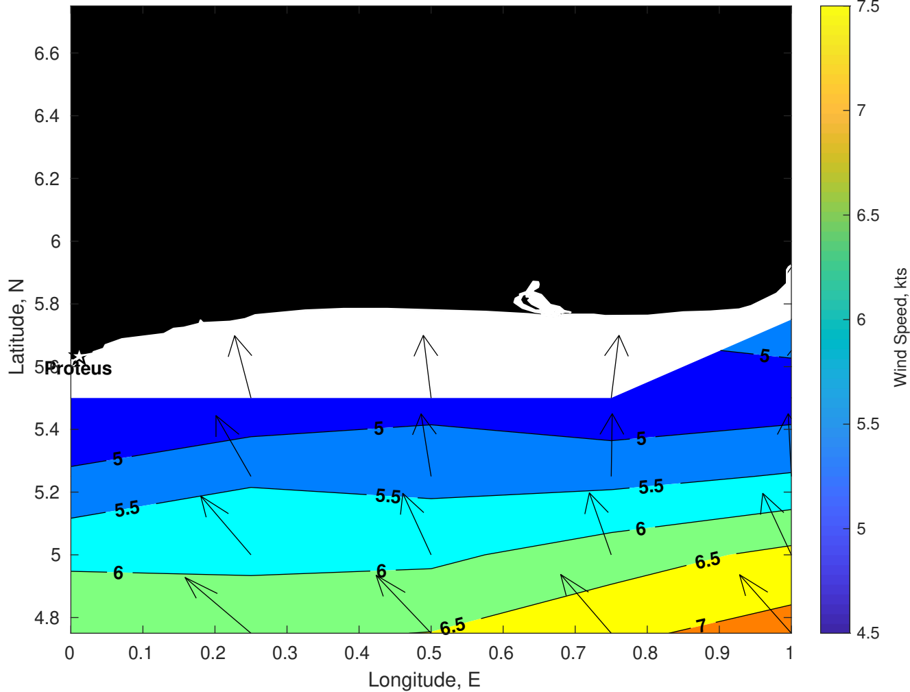
Winds (kts) for Proteus at 11-May-2025 09:00:00
