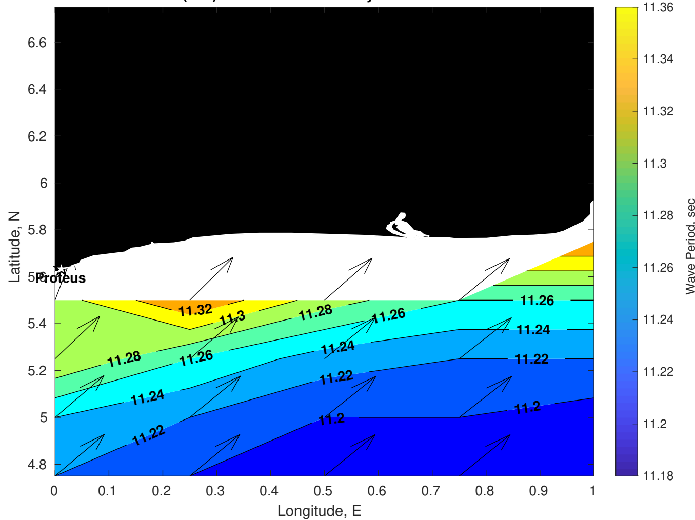
Wave Period (sec) for Proteus at 11-May-2025 09:00:00
