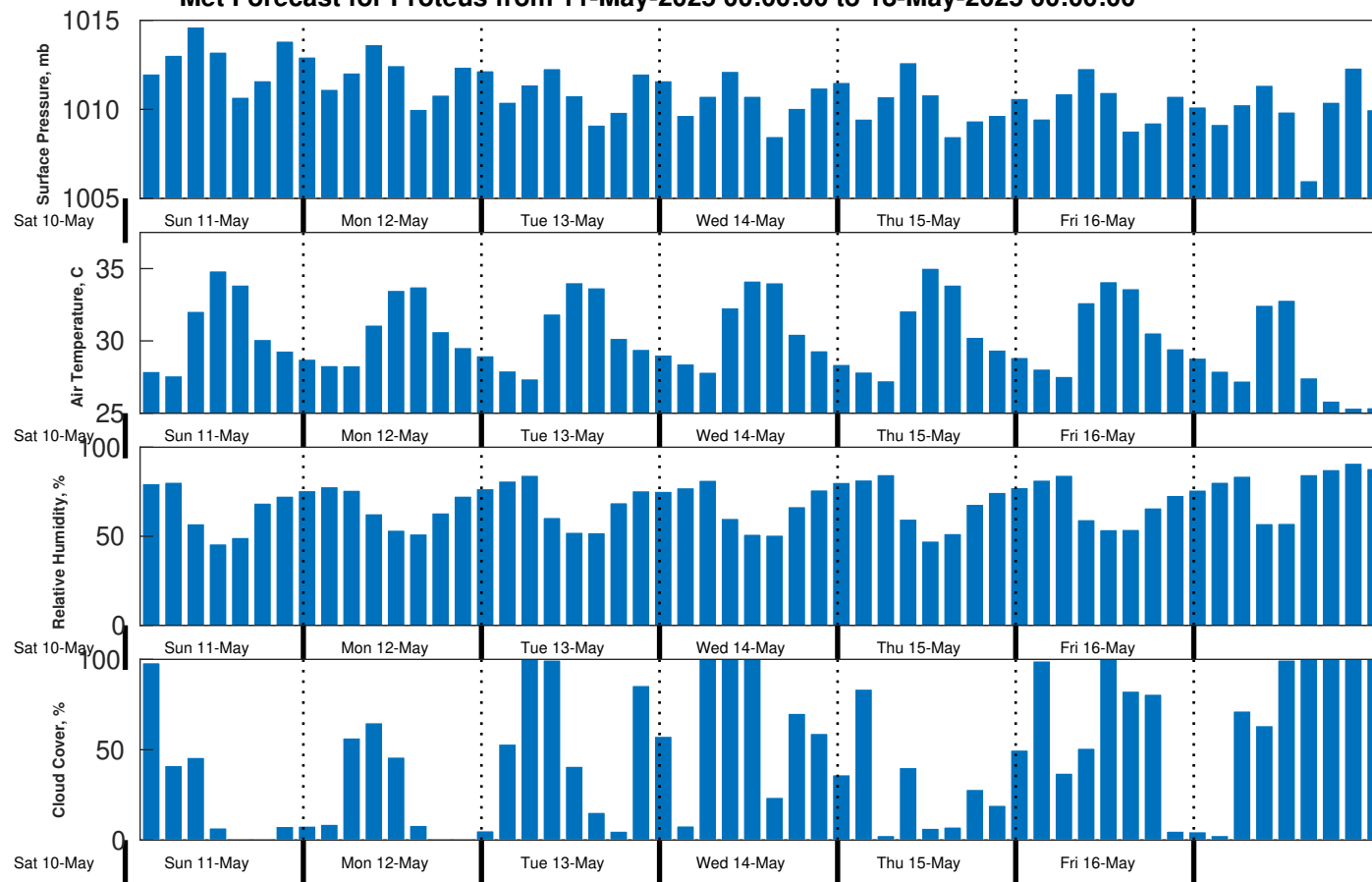
Met Forecast for Proteus from 11-May-2025 00:00:00 to 18-May-2025 00:00:00
