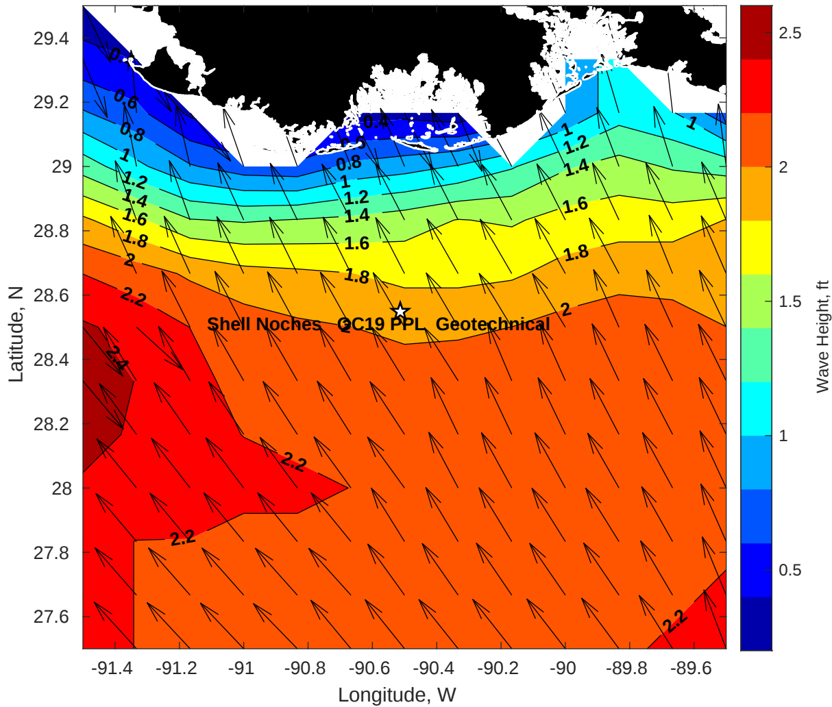
Wave Height (ft) for Shell Noches GC19 PPL Geotechnical at 11-May-2025 09:00:00
