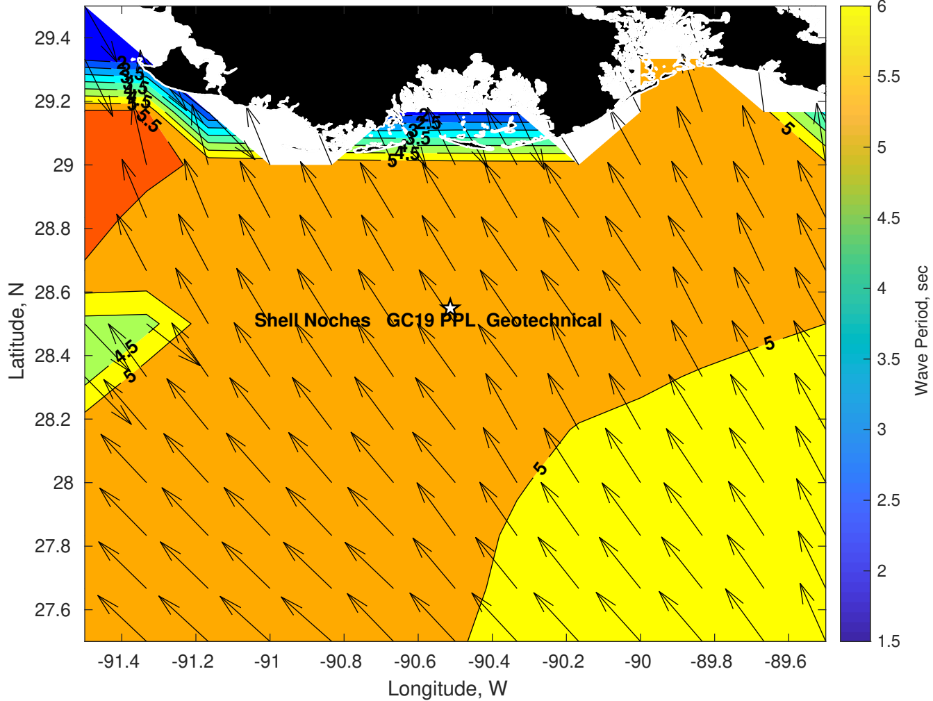
Wave Period (sec) for Shell Noches GC19 PPL Geotechnical at 11-May-2025 09:00:00
