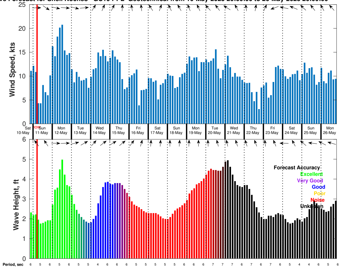
Wind & Wave Forecast for Shell Noches GC19 PPL Geotechnical from 10-May-2025 20:00:00 to 26-May-2025 20:00:00
