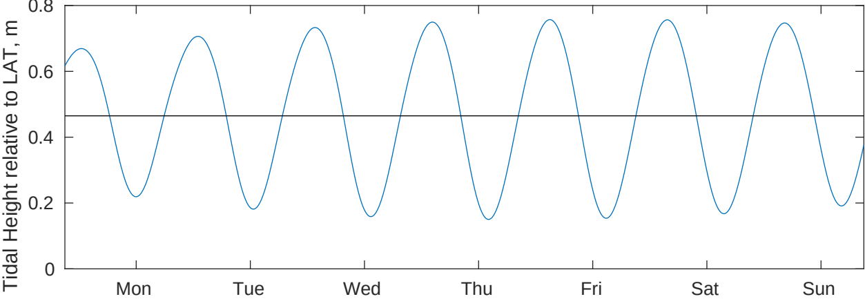
Tidal Currents and Heights for Shell Noches GC19 PPL Geotechnical at 20250511
