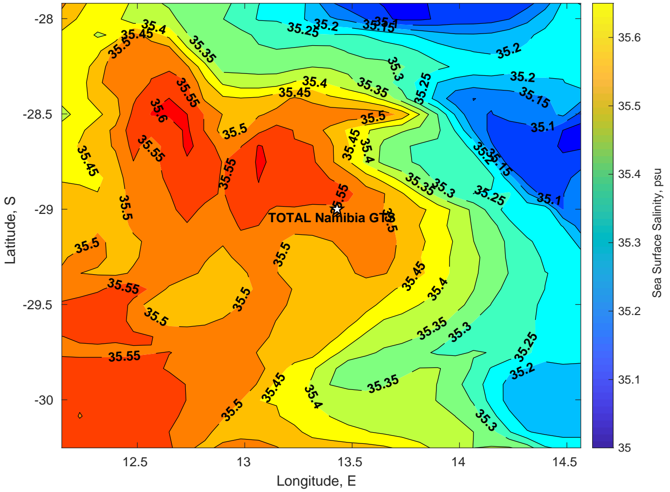
Surface Salinity for TOTAL Namibia GTS at 10-May-2025 00:00:00
