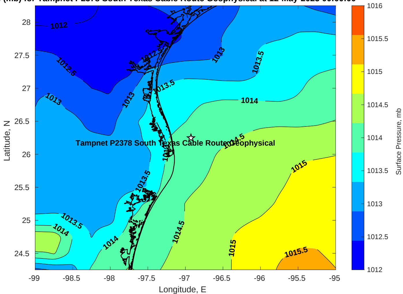
Pressure (mb) for Tampnet P2378 South Texas Cable Route Geophysical at 12-May-2025 00:00:00
