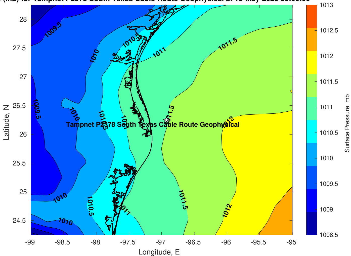
Pressure (mb) for Tampnet P2378 South Texas Cable Route Geophysical at 13-May-2025 00:00:00
