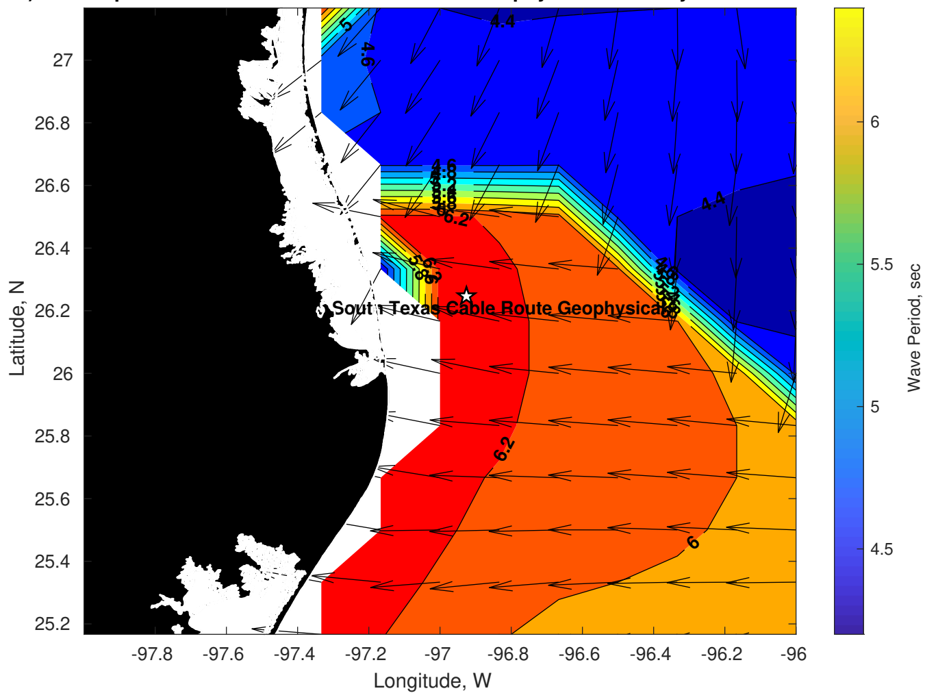
Period (sec) for Tampnet P2378 South Texas Cable Route Geophysical at 11-May-2025 09:00:00
