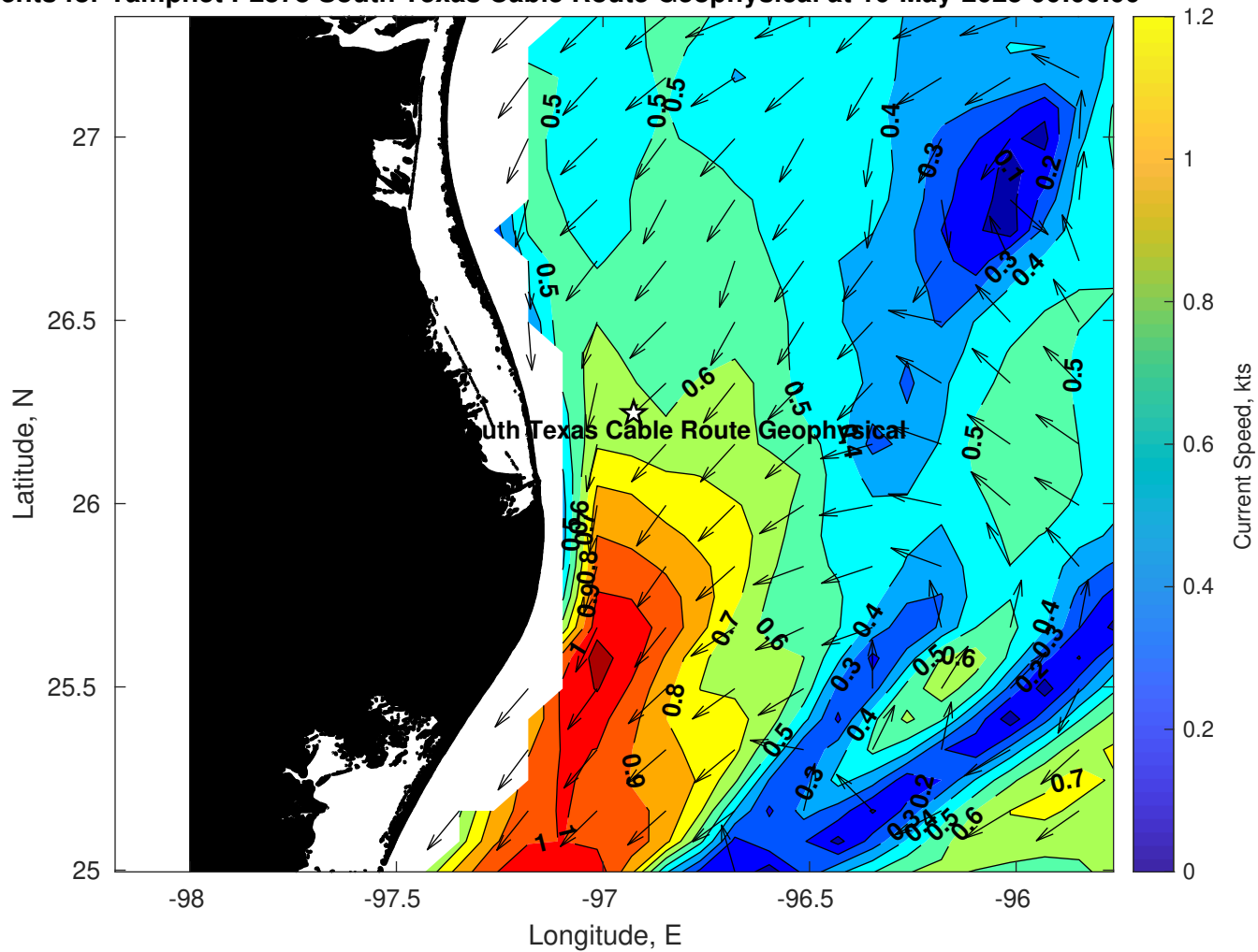
Surface Currents for Tampnet P2378 South Texas Cable Route Geophysical at 10-May-2025 00:00:00
