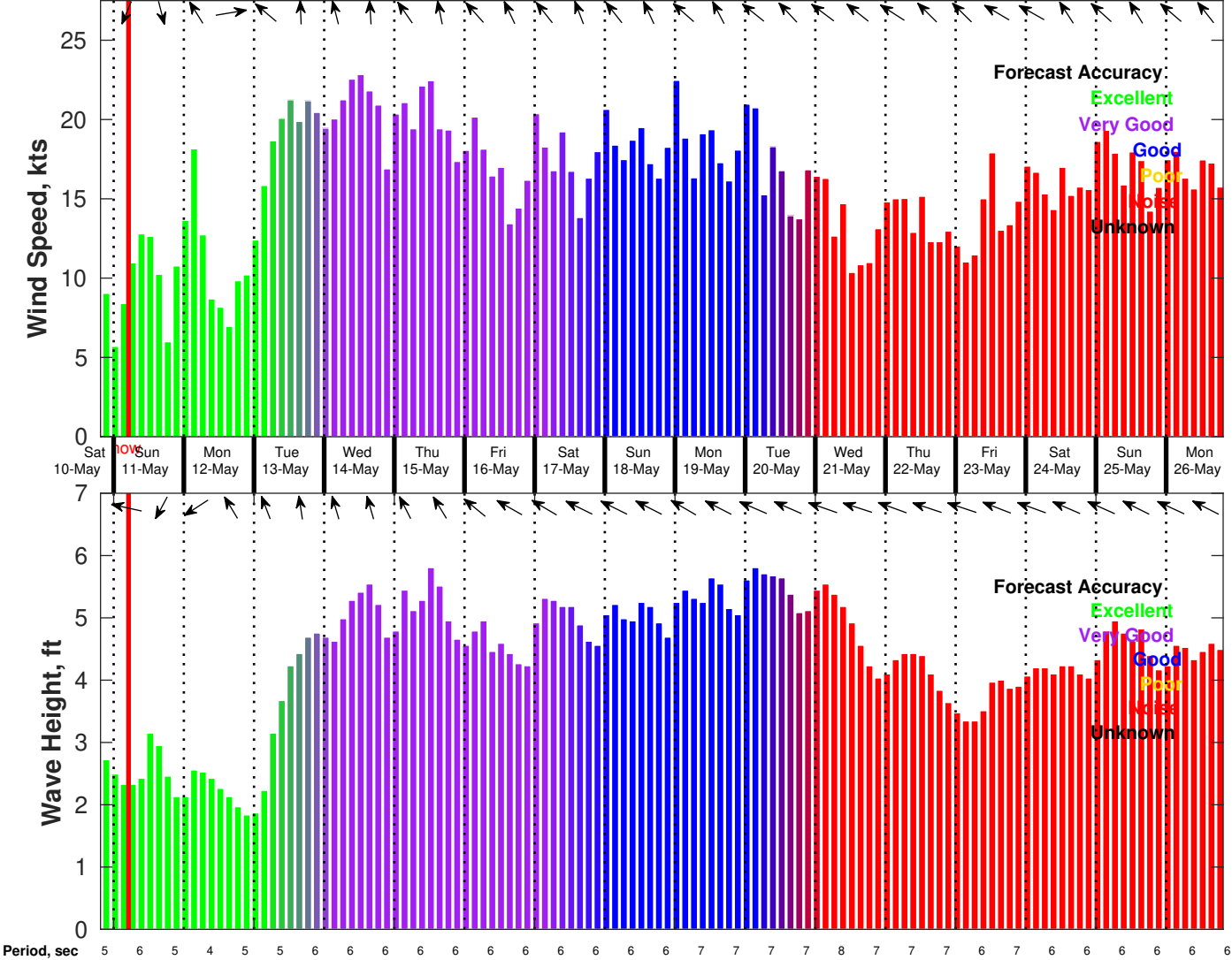
Wind & Wave Forecast for Tampnet P2378 South Texas Cable Route Geophysical from 10-May-2025 20:00:00 to 26-May-2025 20:00:00
