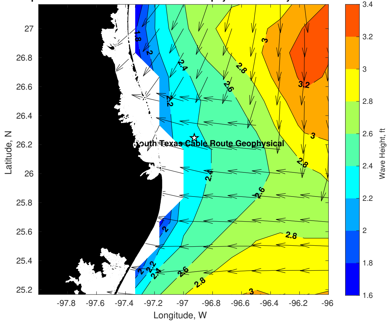
Wave Height (ft) for Tampnet P2378 South Texas Cable Route Geophysical at 11-May-2025 09:00:00
