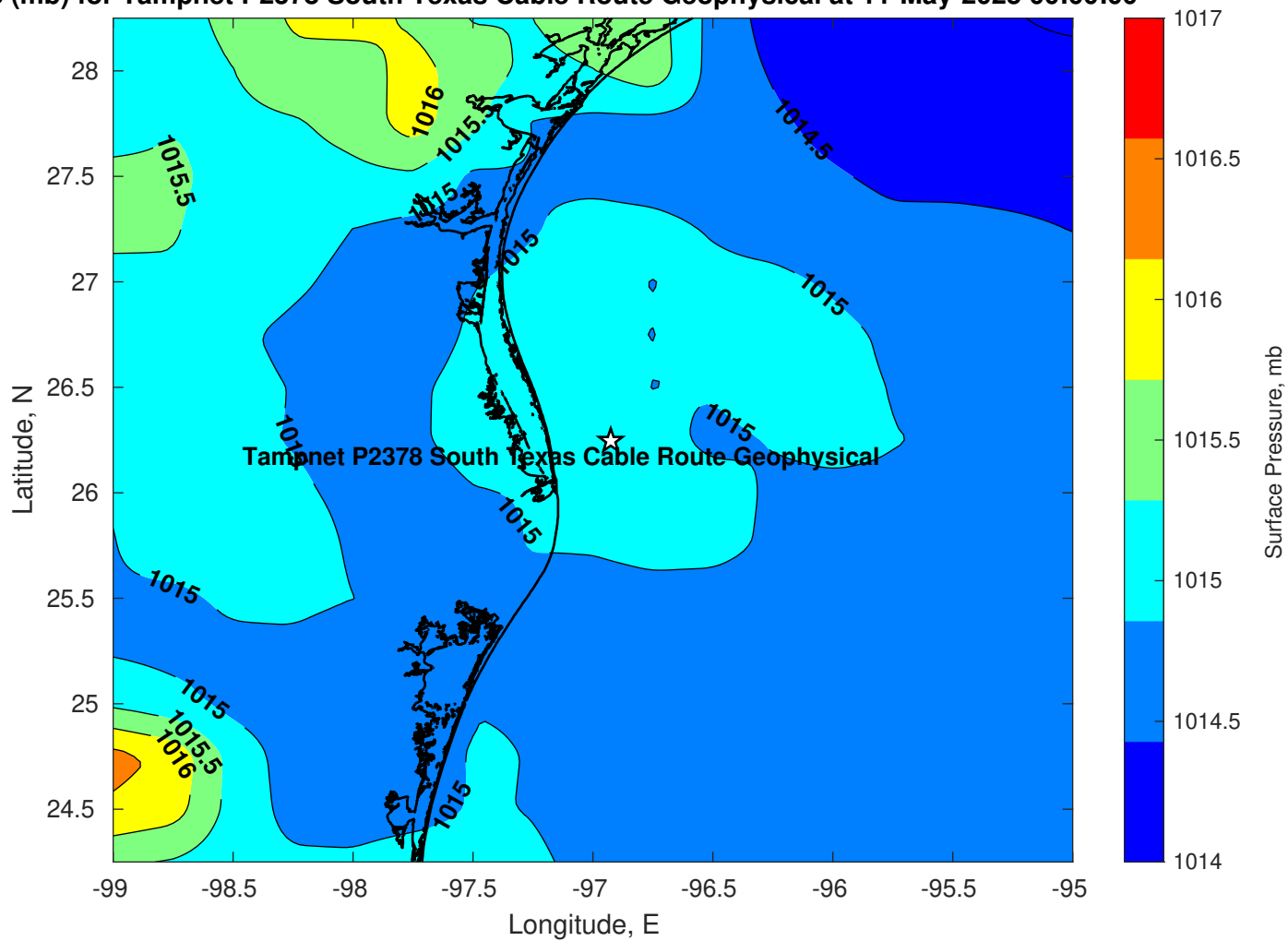
Pressure (mb) for Tampnet P2378 South Texas Cable Route Geophysical at 11-May-2025 00:00:00
