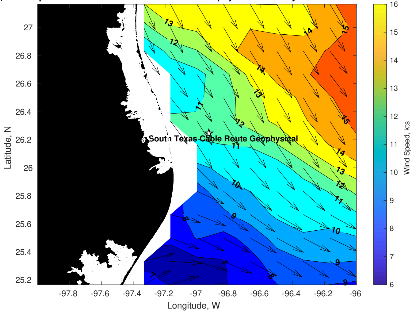
Winds (kts) for Tampnet P2378 South Texas Cable Route Geophysical at 11-May-2025 09:00:00
