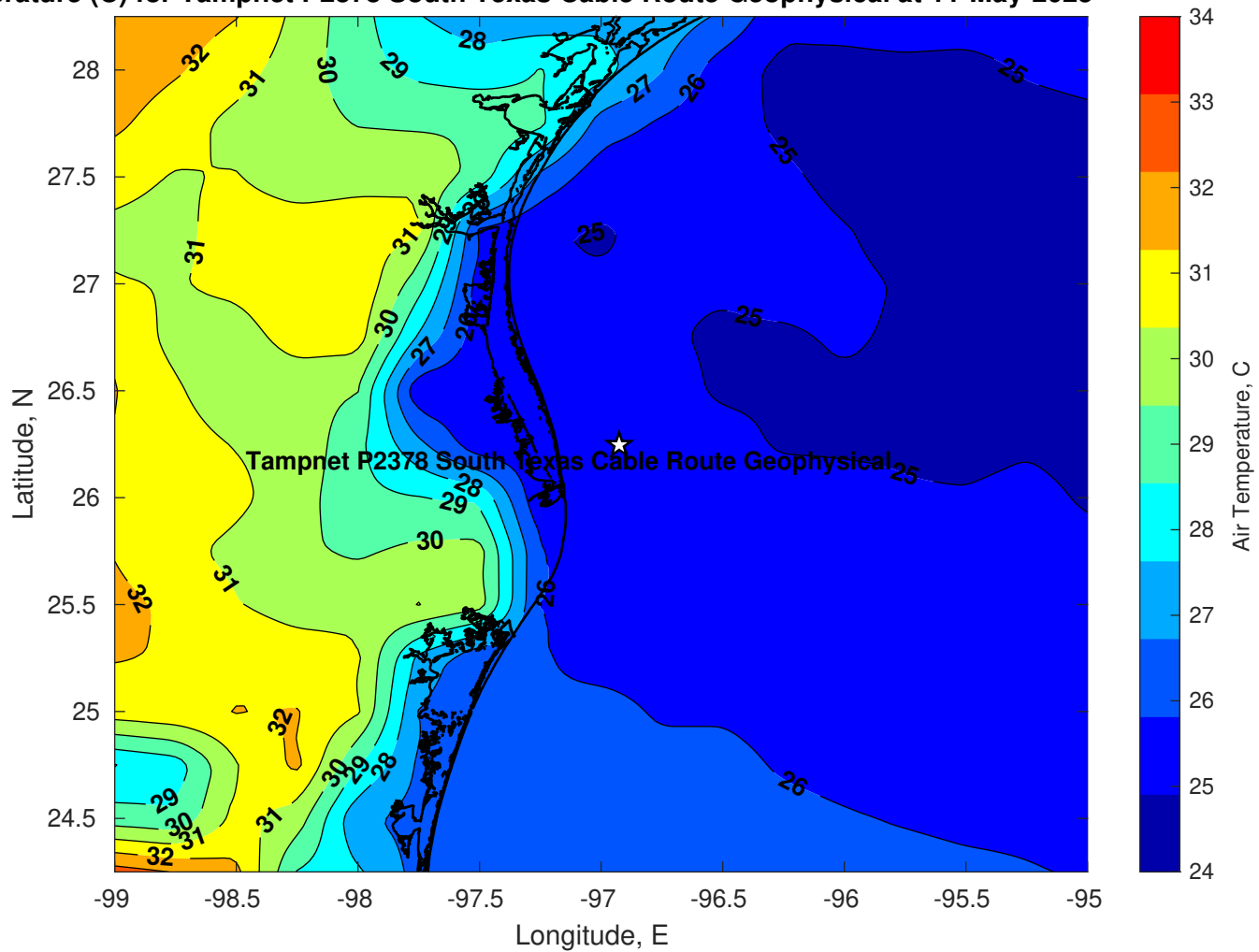
Air Temperature (C) for Tampnet P2378 South Texas Cable Route Geophysical at 11-May-2025
