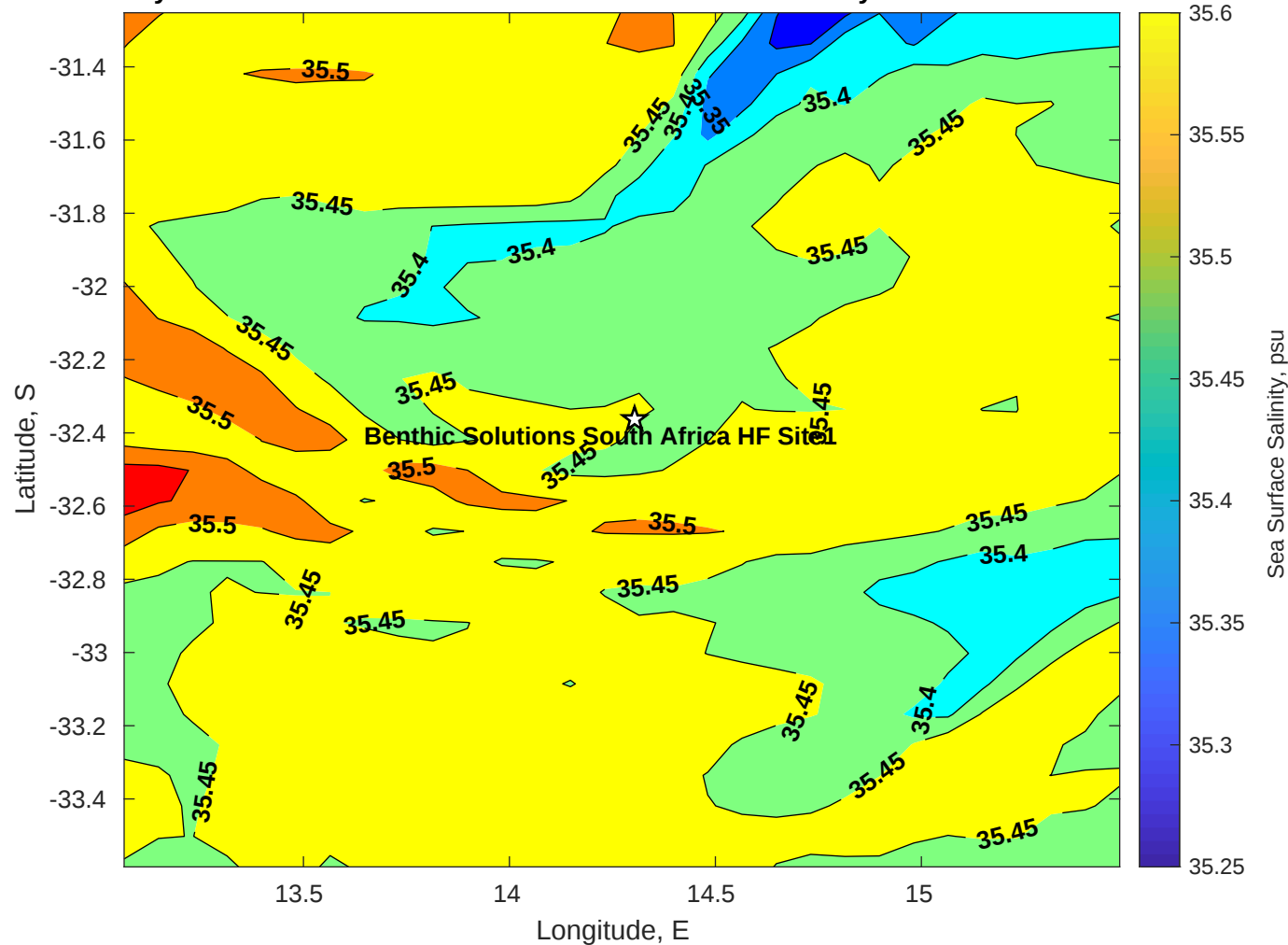
Surface Salinity for Benthic Solutions South Africa HF Site1 at 11-May-2025 00:00:00
