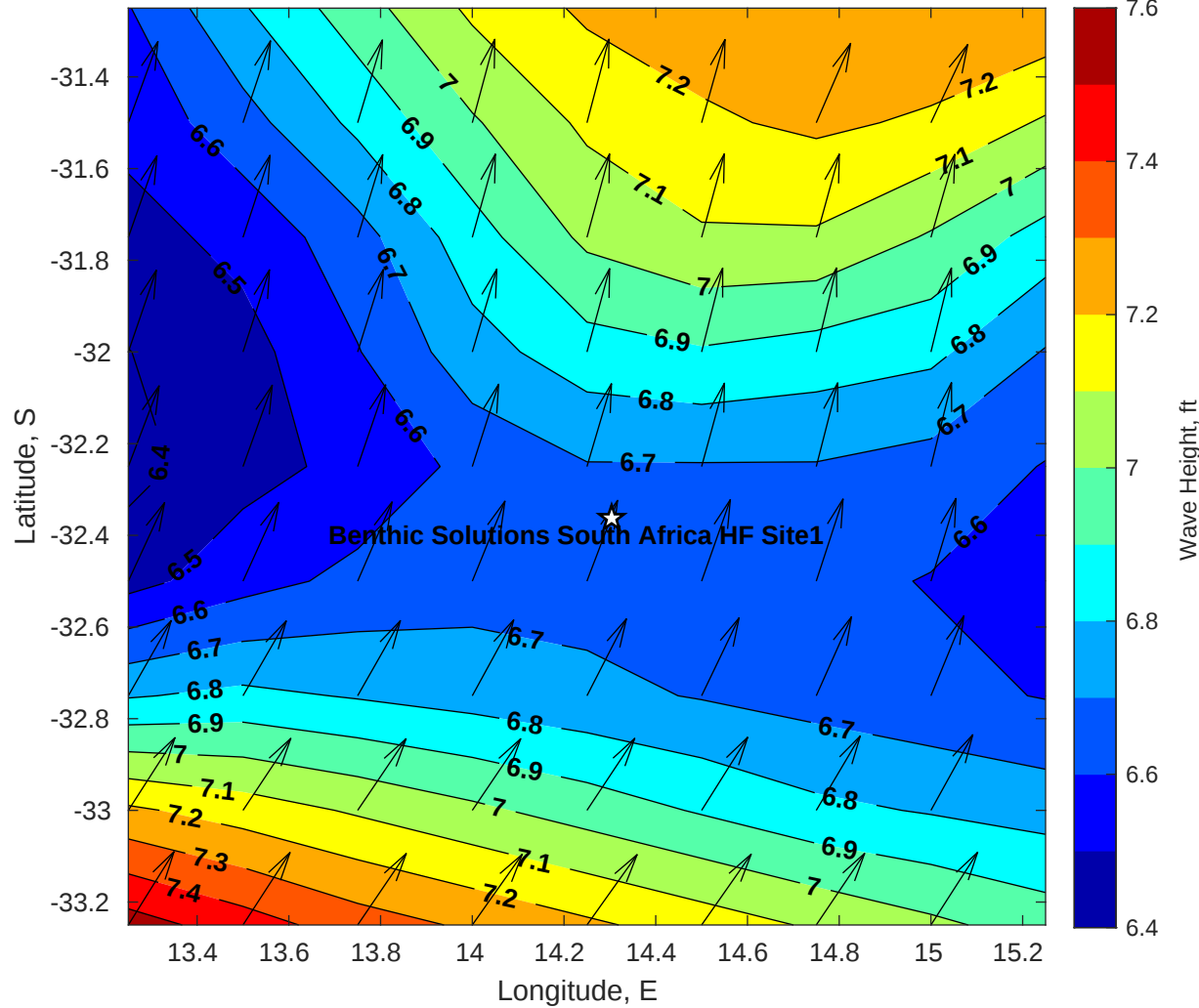
Wave Height (ft) for Benthic Solutions South Africa HF Site1 at 12-May-2025 09:00:00
