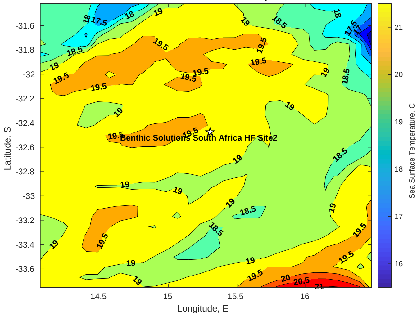
SST for Benthic Solutions South Africa HF Site2 at 11-May-2025 00:00:00
