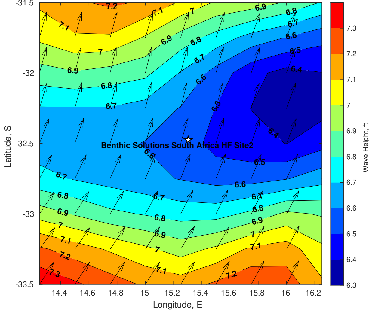
Wave Height (ft) for Benthic Solutions South Africa HF Site2 at 12-May-2025 09:00:00
