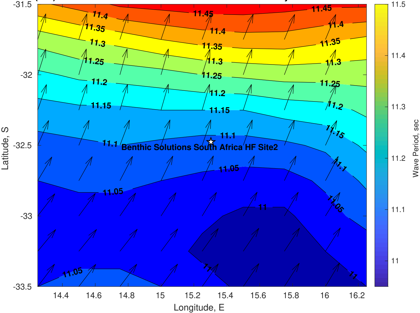
Wave Period (sec) for Benthic Solutions South Africa HF Site2 at 12-May-2025 09:00:00
