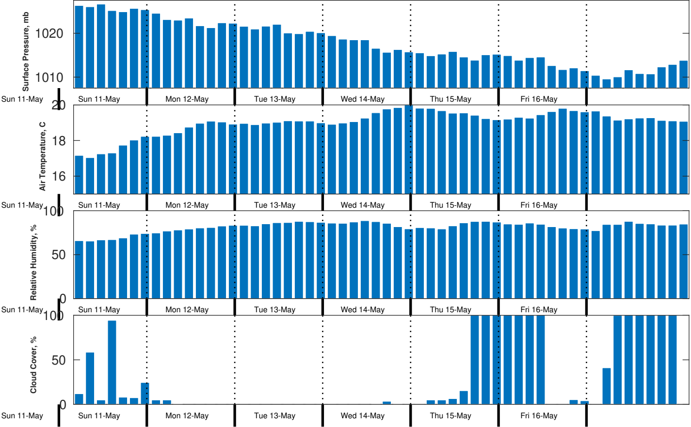
Met Forecast for Benthic Solutions South Africa HF Site2 from 12-May-2025 00:00:00 to 19-May-2025 00:00:00
