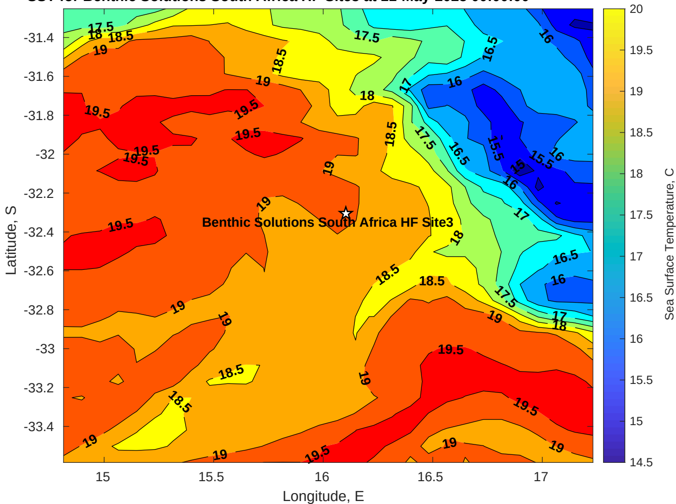
SST for Benthic Solutions South Africa HF Site3 at 11-May-2025 00:00:00
